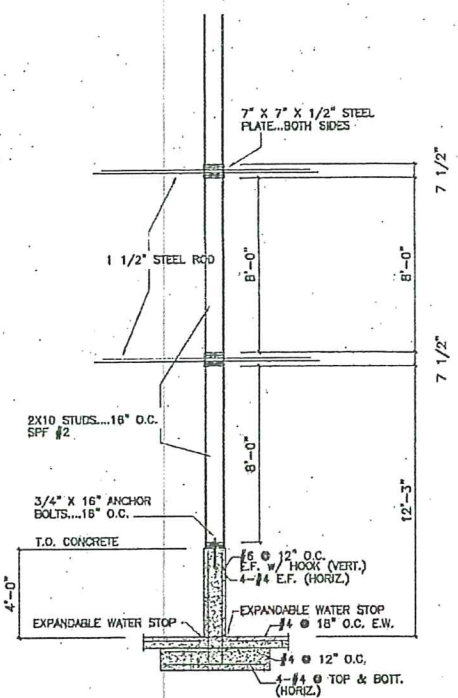
(A) WALL DETAIL SCALE: 1/4" = 1'-0"
