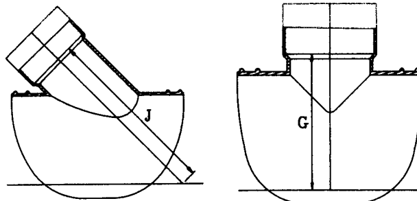
45° SADDLE WYE SADDLE TEE FIG. X3.7 Saddles
