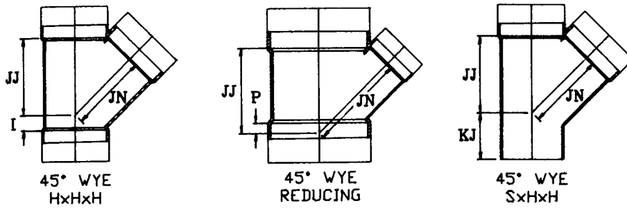
FIG. X3.4 Wyes
