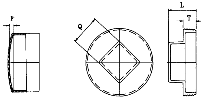
FIG. X3.8 Caps/Plugs
