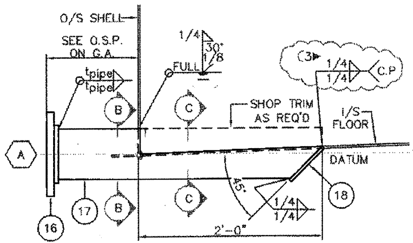
ASSEMBLY 3-D
