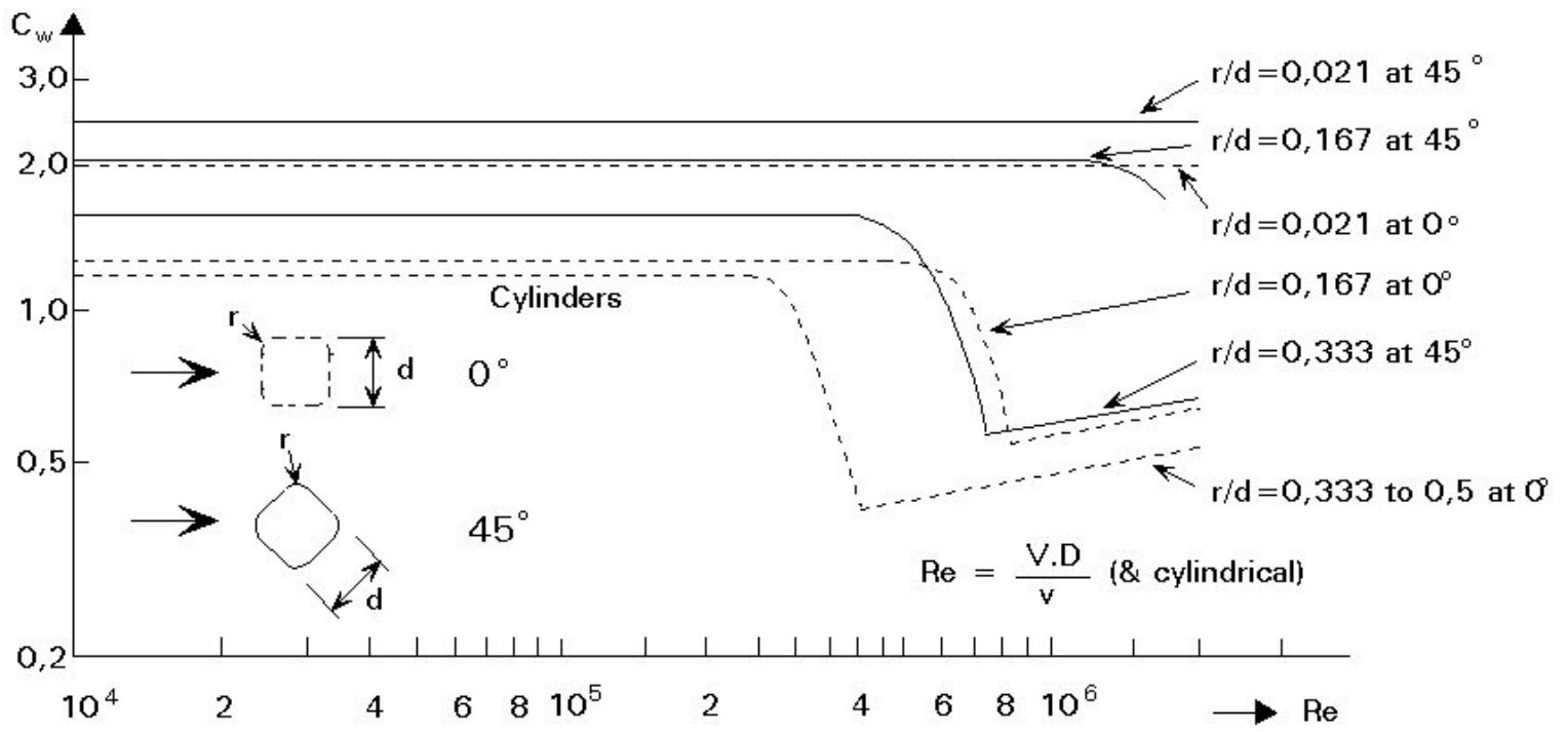
Figure 4 Drag coefficient curves for single square section (smooth surface) members with various corner radii depending on Reynold's number
