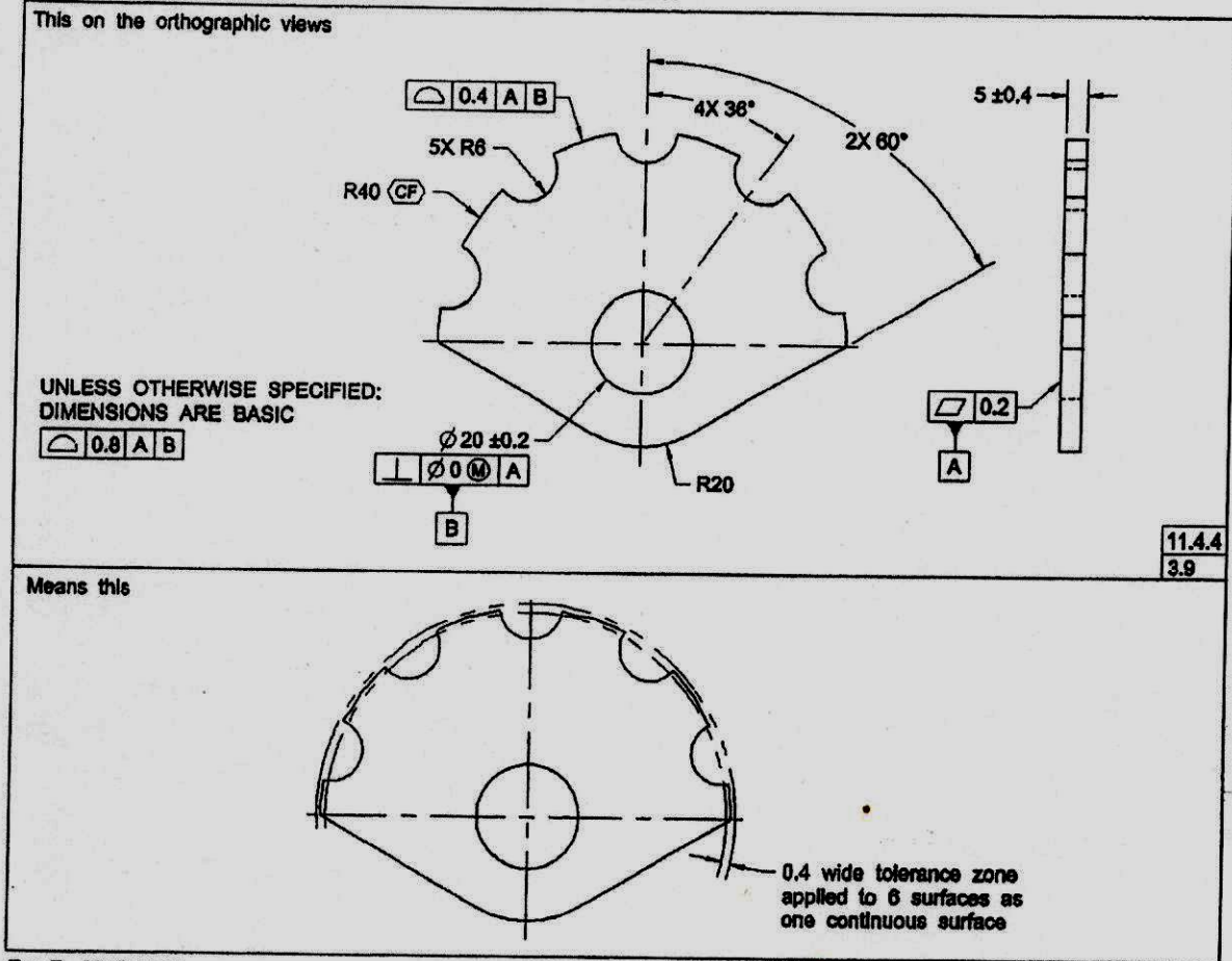
Fig. 11-23 Continuous Feature Symbol Application in a Profile Tolerance
