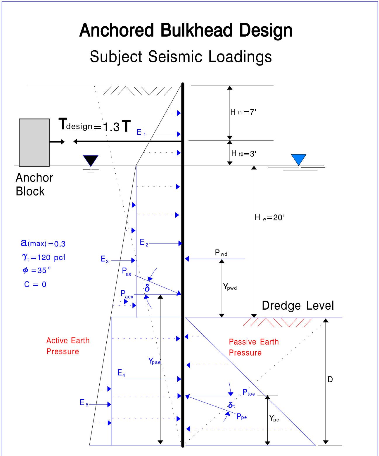
Figure 32 Example of Anchored Sheet Pile Wall Design
