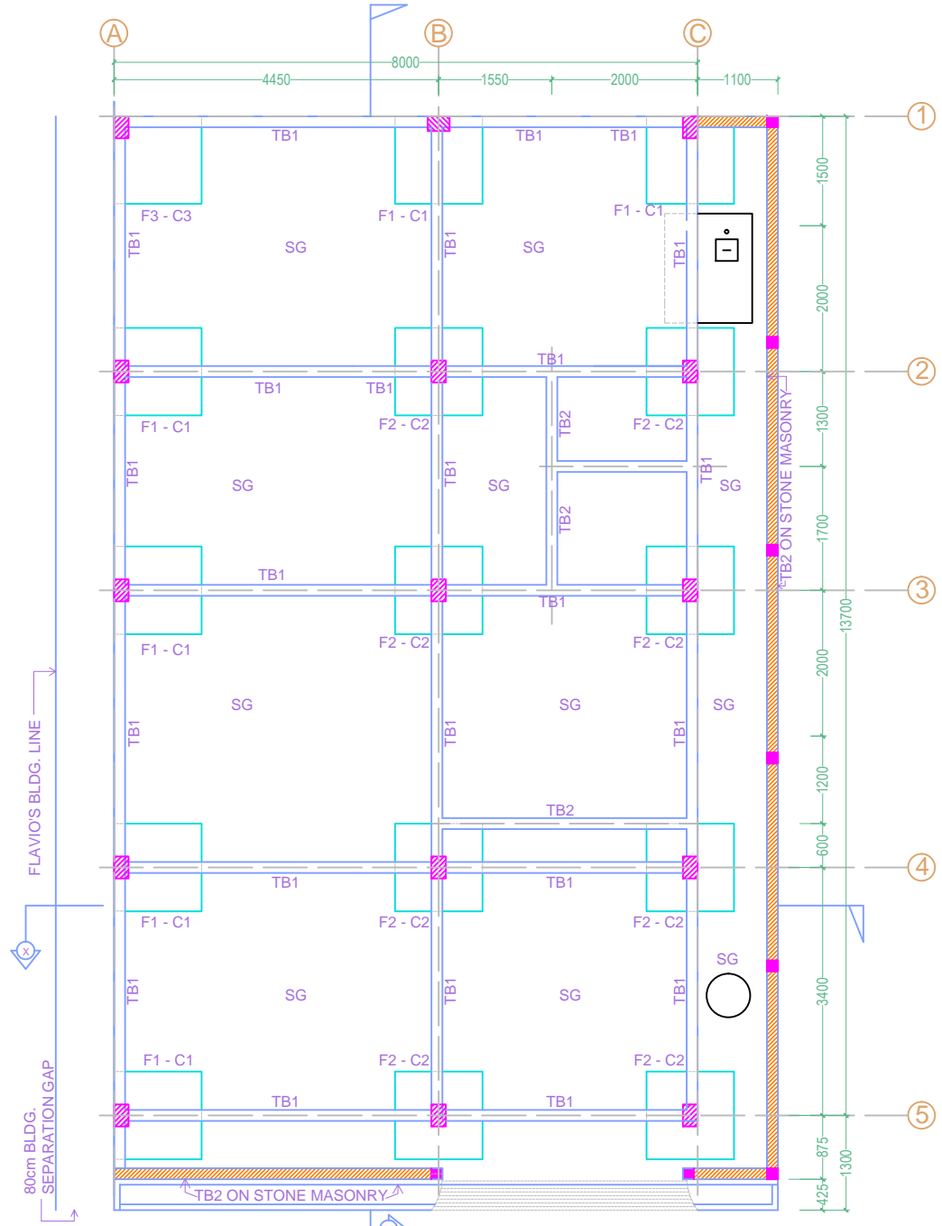
S FOUNDATION PLAN SCALE 1:100 MTS
