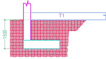
S ECCENTRIC FOOTING (F3 - C3) SCALE 1:100 MTS
