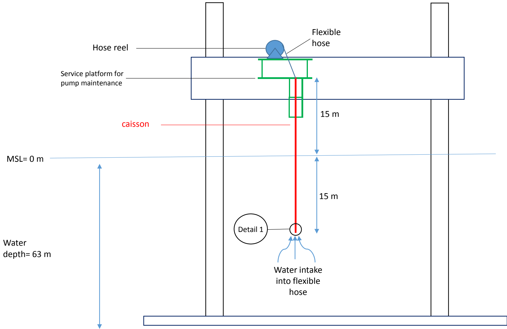
ELEVATION VIEW OF MOPU
