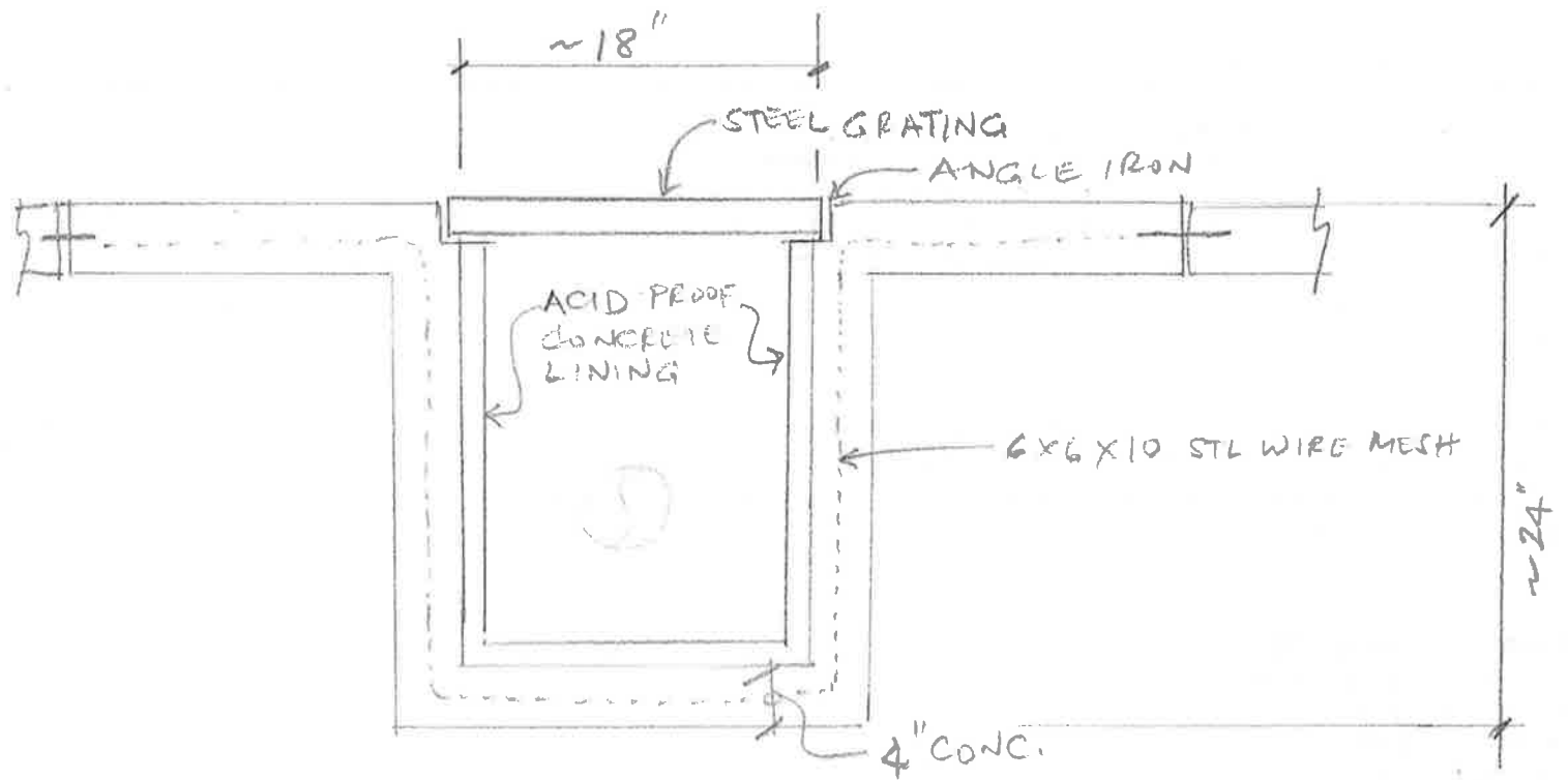
CROSS SECT-TRENCH CONFIGURATION WHEN IT WAS NEW
