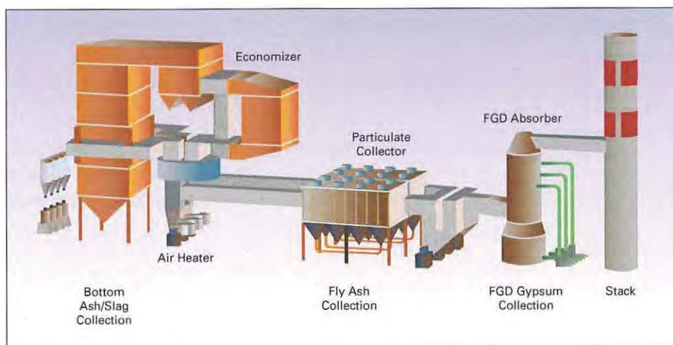
Figure 1. Typical power plant layout showing location of fly ash and bottom ash collection.
