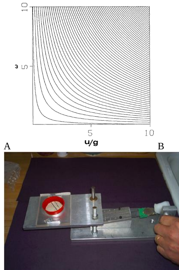
Figure 10. A. Keller's (1986) curves separating coin-toss solutions for heads and tails for a coin tossed from elevation 0 with initial upward velocity u and angular velocity \omega . B. Diaconis et al.'s (2007) coin-tossing device
