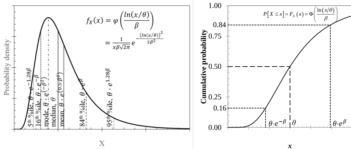
Figure 3. Left: Lognormal probability density function. Right: Lognormal cumulative distribution function
