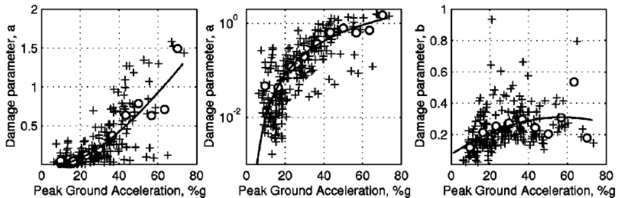
Figure 14. Regression analysis of damage to woodframe buildings in the 1994 Northridge earthquake (Wesson et al. 2006)
