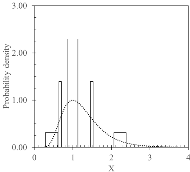
Figure 24. 5-point moment matching for a lognormal probability distribution
