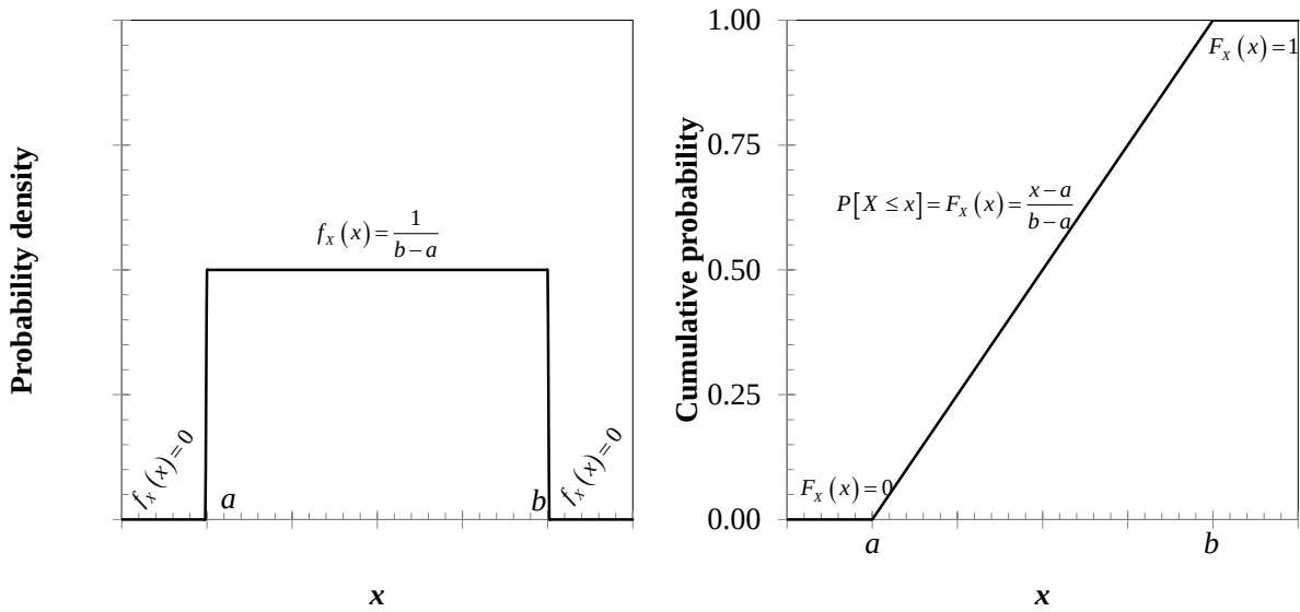
Figure 5. Left: Uniform probability density function. Right: Uniform cumulative distribution function
