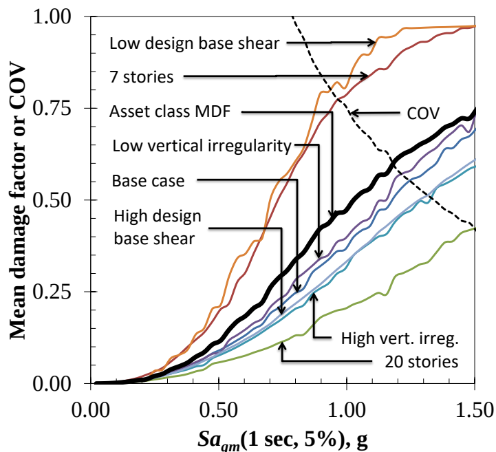
Figure 17. Example analytical vulnerability function for highrise post-1980 reinforced concrete moment frame office building in the Western United States (Kazantzi et al. 2013)
