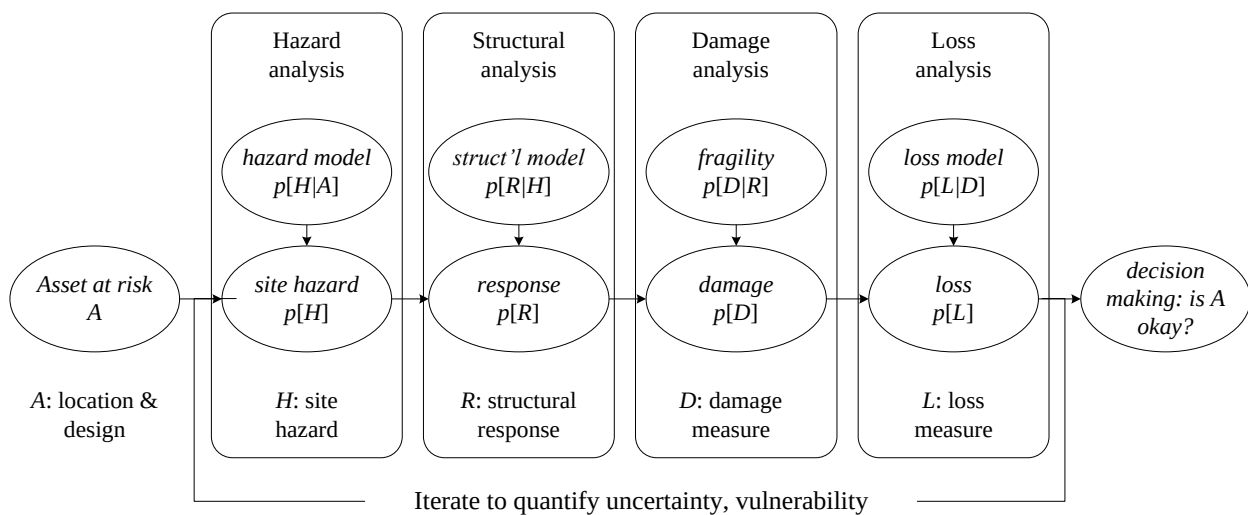
Figure 15. Analytical methods for estimating seismic vulnerability of a single asset (Porter 2003).
