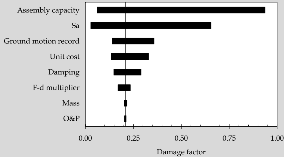
Figure 28. A sample tornado diagram that depicts how the earthquake-induced repair cost for a particular building is affected by various model parameters (Porter et al. 2002).
