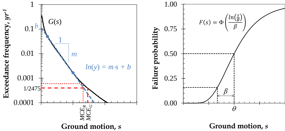
Figure 20. Calculating failure rate with hazard curve (left) and fragility function (right)
