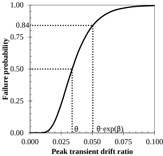
Figure 25. Exercise 1 fragility function
