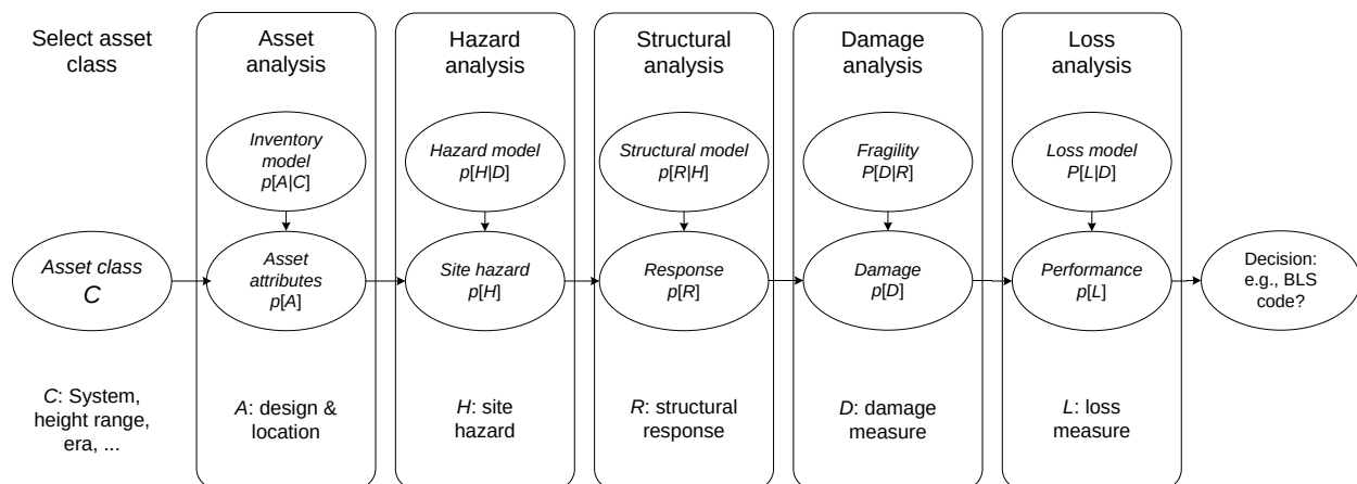
Figure 16. Accounting for variability in design within the asset class, one can extend PBEE to estimate seismic vulnerability of an asset class
