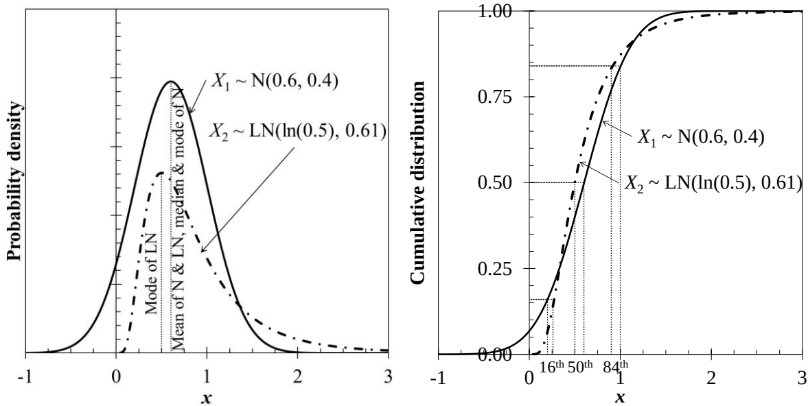
Figure 4. Normal and lognormal distributions with the same mean and standard deviation
