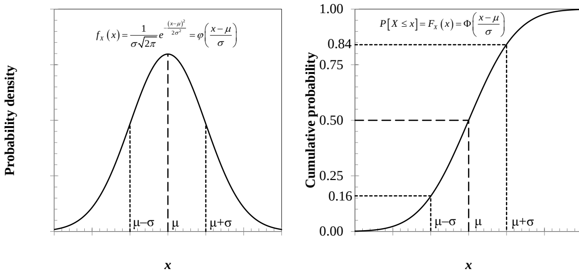
Figure 2. Left: Gaussian probability density function. Right: Gaussian cumulative distribution function
