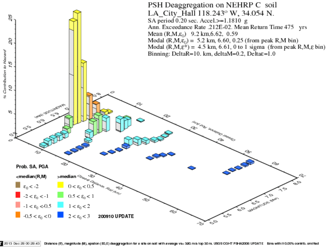
Figure 26. 475-year (10%/50-year) Sa(0.2 sec, 5%) hazard deaggregation at LA City Hall
