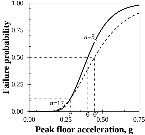
Figure 12. Increasing beta and adjusting theta to account for under-representative samples
