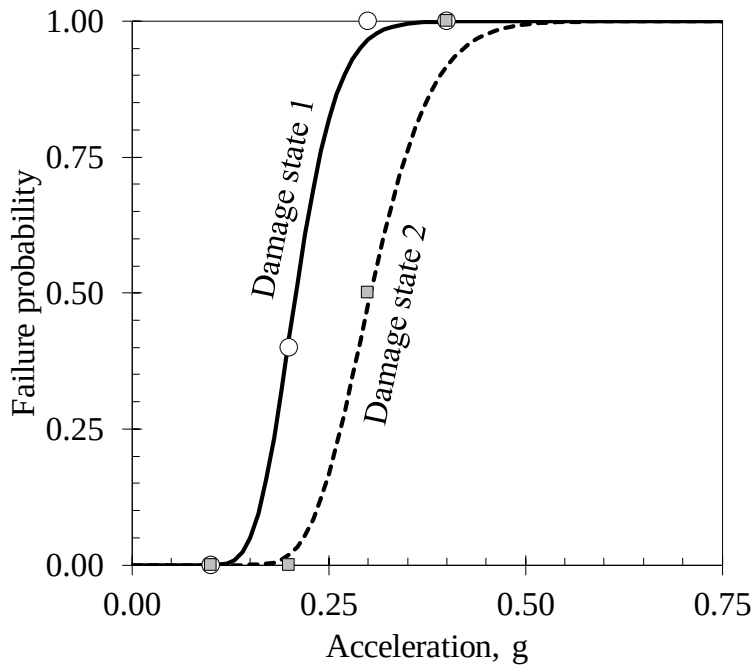
Figure 13. Illustration of maximum likelihood estimation of lognormal fragility functions with type-B data and multiple sequential damage states, solution
