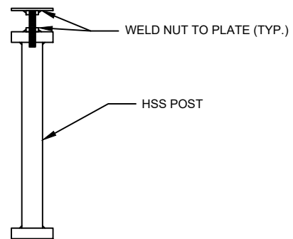
DETAIL P1
