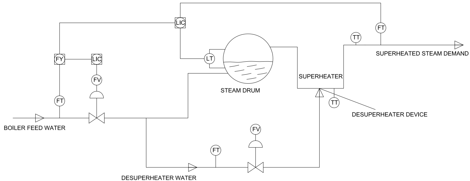
CASE No 1 WHERE DESUPERHEATER WATER PIPE COMES FROM BOILER FEED WATER AND IT IS AFTER FV
