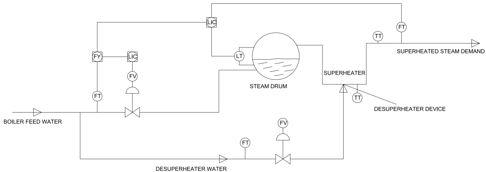
CASE No 2 WHERE DESUPERHEATER WATER PIPE COMES FROM BOILER FEED WATER AND IT IS BEFORE FV AND FT
