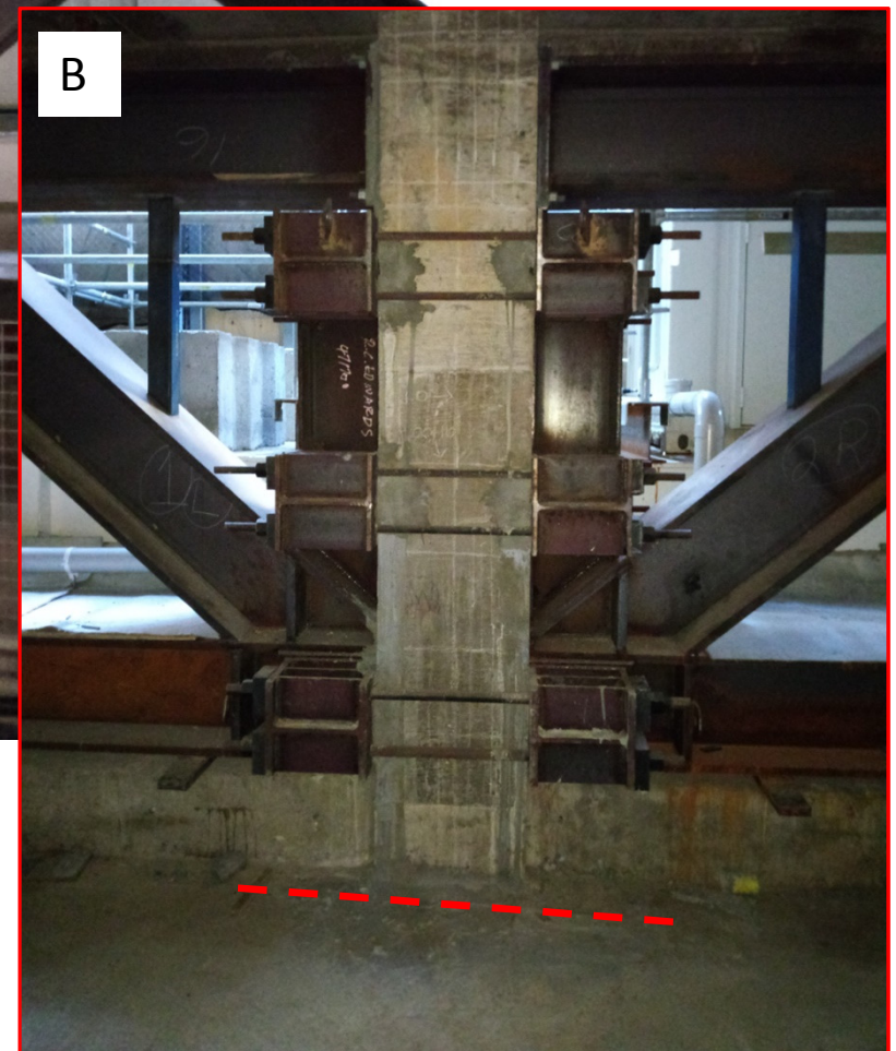
Figure 1. A – photograph of truss from inside of building at first floor level. B – close-up photograph of shear-key
