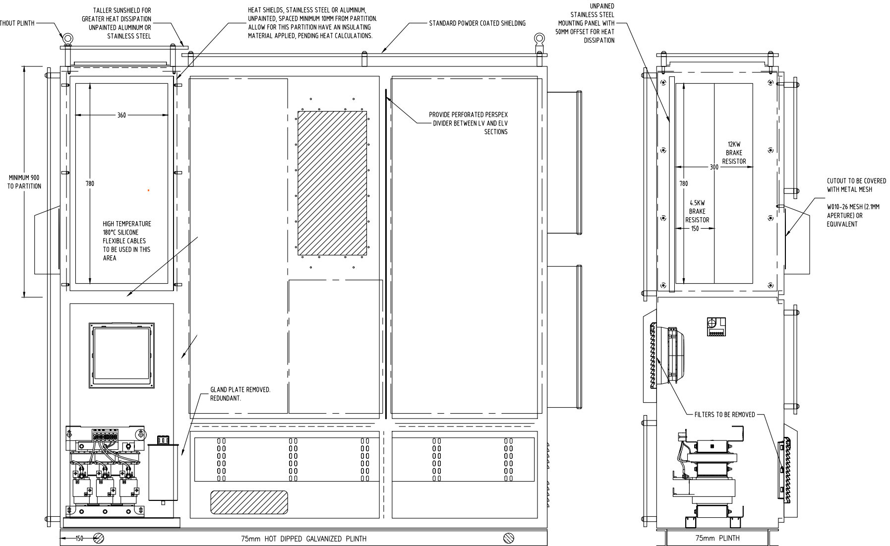
FRONT VIEW LESS DOORS
