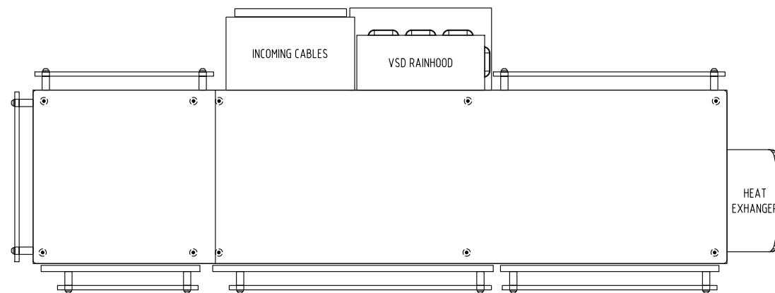
TOP VIEW
