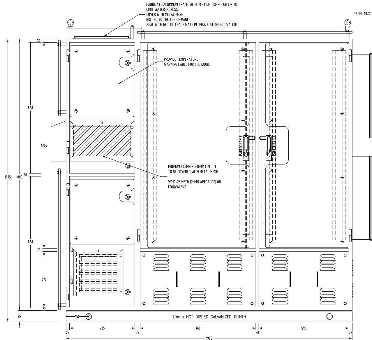
FRONT VIEW
