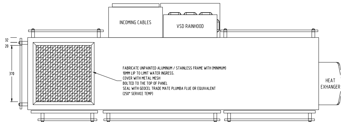
TOP VIEW WITH ROOF REMOVED
