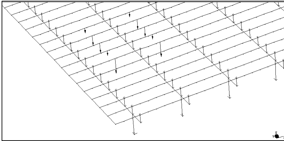
Figure 1: Downstand grillage model detail
