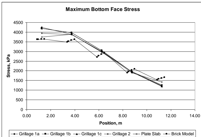
Figure 8: Maximum Bottom Face Stress
