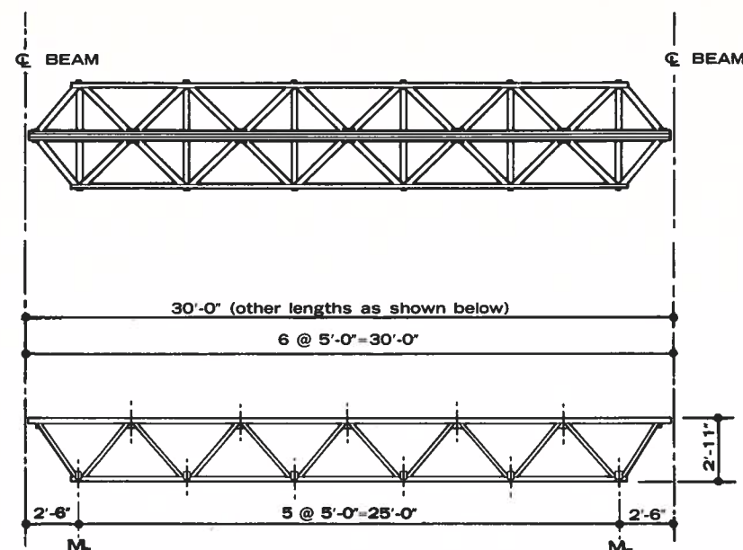
SPACE TRUSS ELEVATION 30' SPACE TRUSS SHOWN Scale: 1/8"=1'-0"
