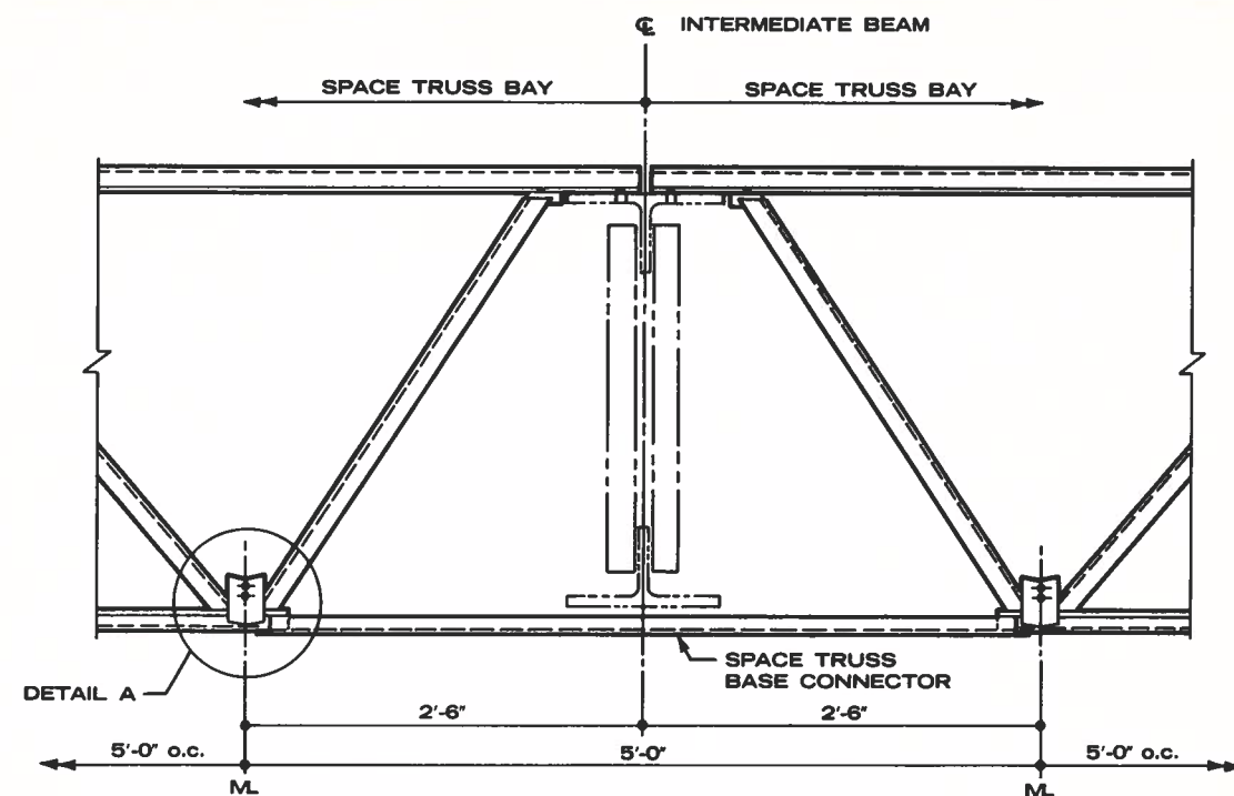
SPACE TRUSS BASE CONNECTOR AT INTERMEDIATE BEAM Scale: \frac{3}{4} "=1'-0"
