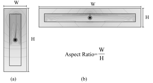
Fig. 4. Troughs flush with the soil showing the isotherms. (a) Small aspect ratio 0.22. (b) Large aspect ratio 2.25.
