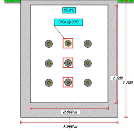
Fig. 1. Example of unfilled trough installation with lid flush with the surface.
