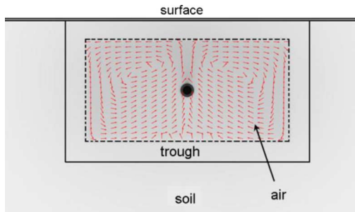
Fig. 2. Unfilled trough with lid flush with the soil surface.
