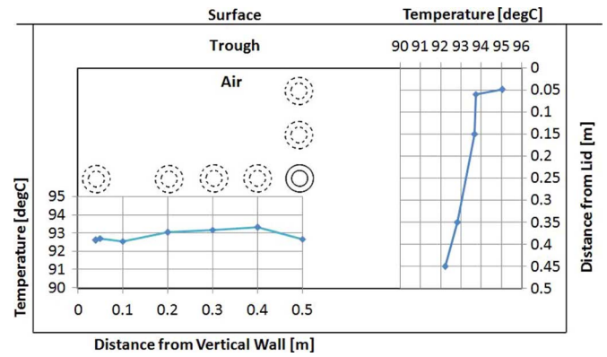
Fig. 6. Horizontal and vertical cable position versus maximum conductor temperature at the steady state.
