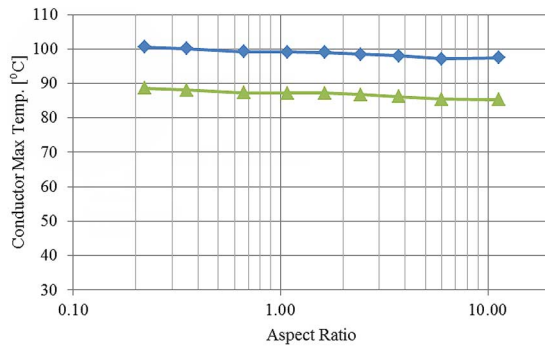
Fig. 5. Aspect ratio versus maximum conductor temperature for ambient temperatures of 45 °C and 32 °C.
