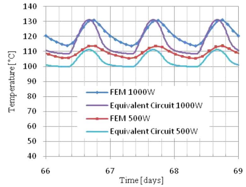
Fig. 9. Temperature swing within the trough due to solar radiation from FEM and the thermal circuit.
