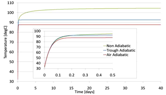
Fig. 3. Plot of temperature versus time for air adiabatic, trough adiabatic, and nonadiabatic conditions.
