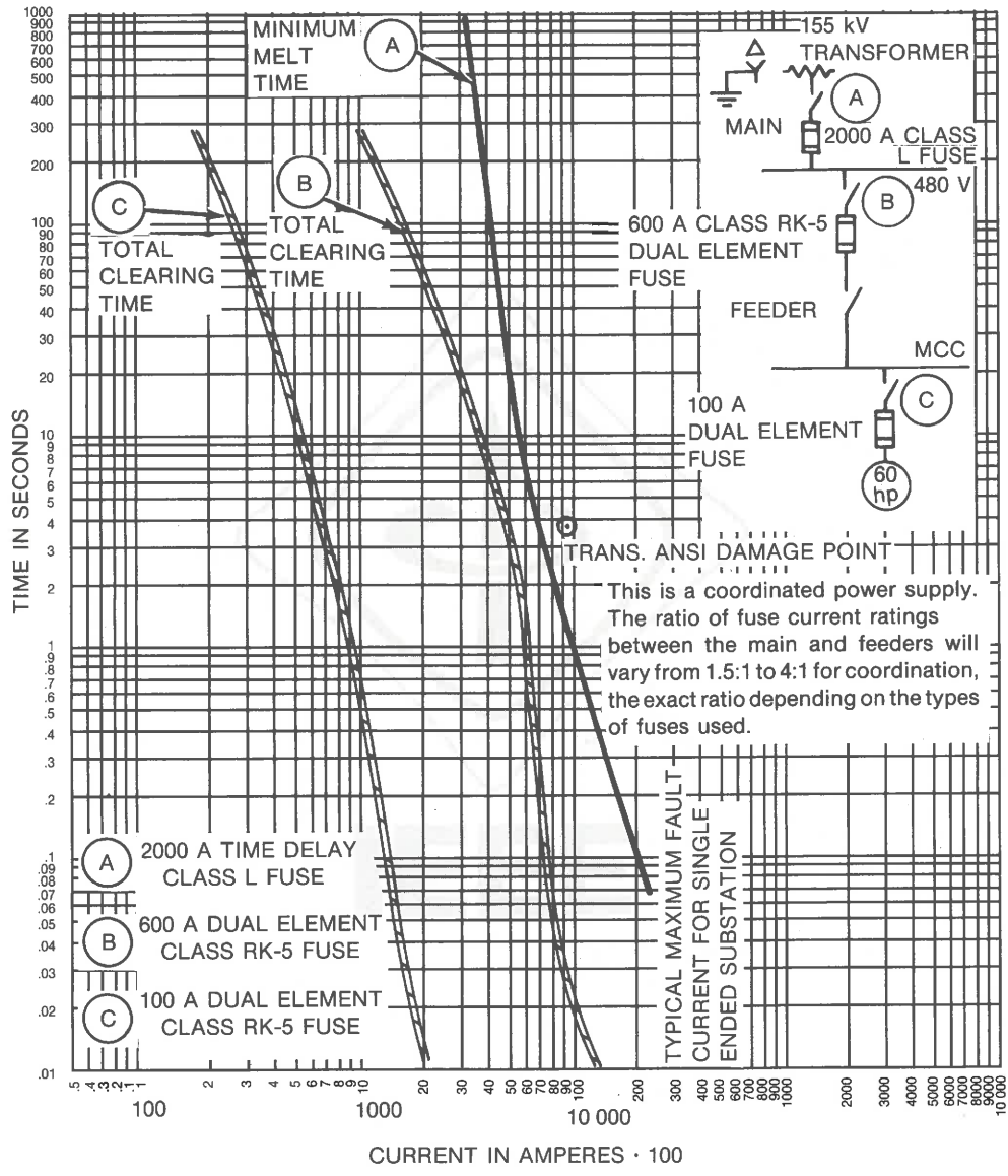
Fig 246 Ground-Fault Time-Current Characteristic Curves
