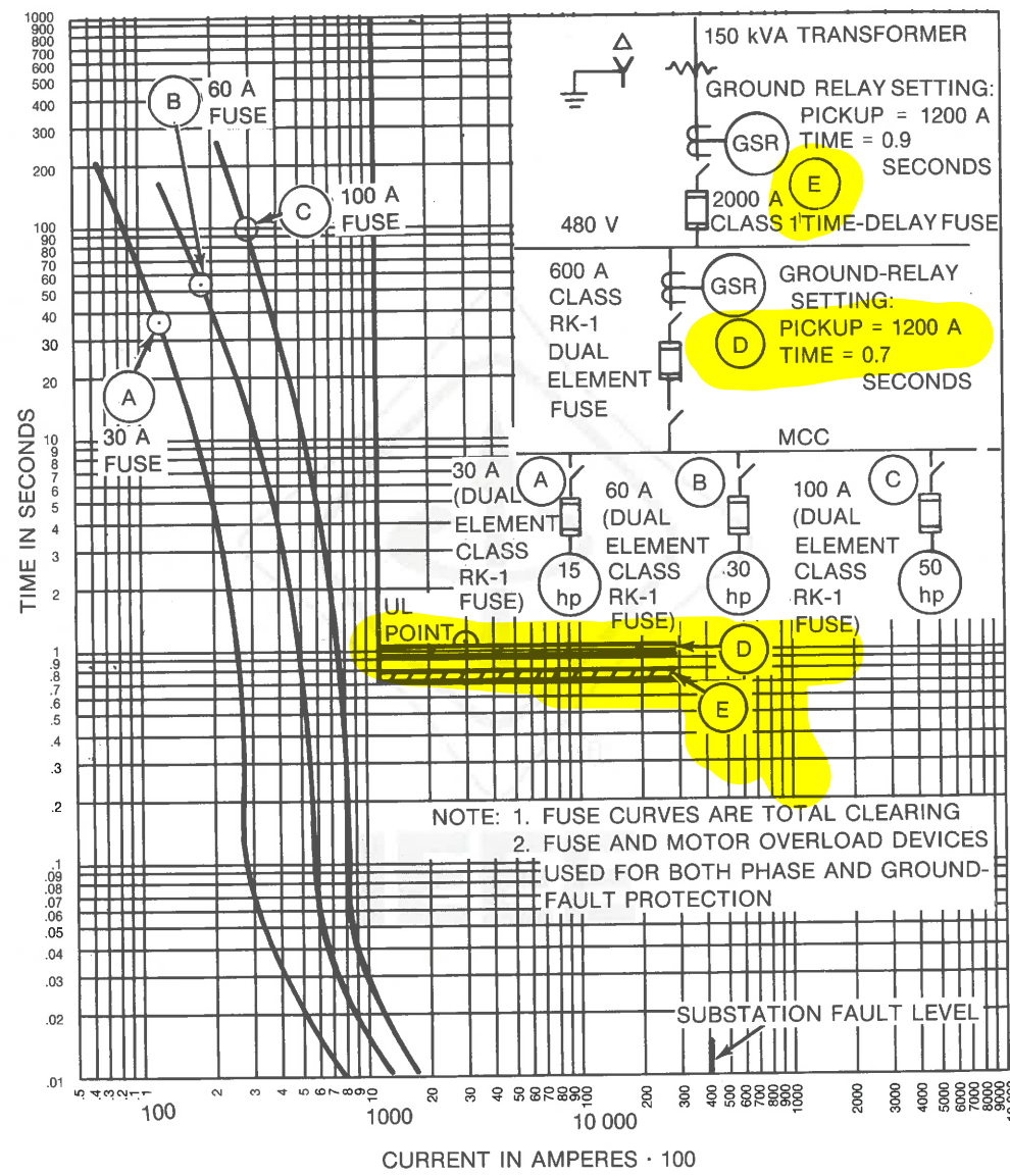
Fig 245 Ground-Fault Time-Current Characteristic Curves
