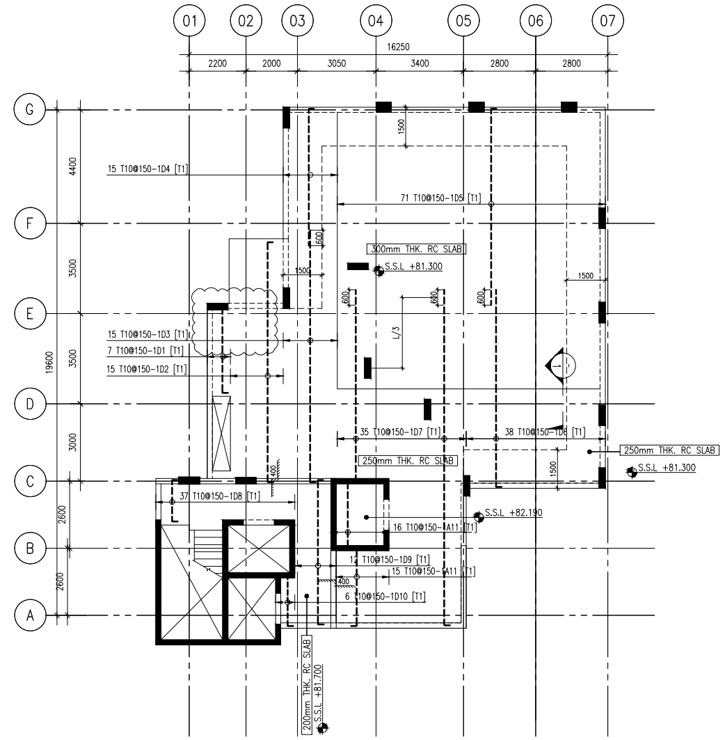
REINFORCEMENT DETAILS OF SLAB AT ROOF LEVEL TOP - T1 SCALE 1:100
