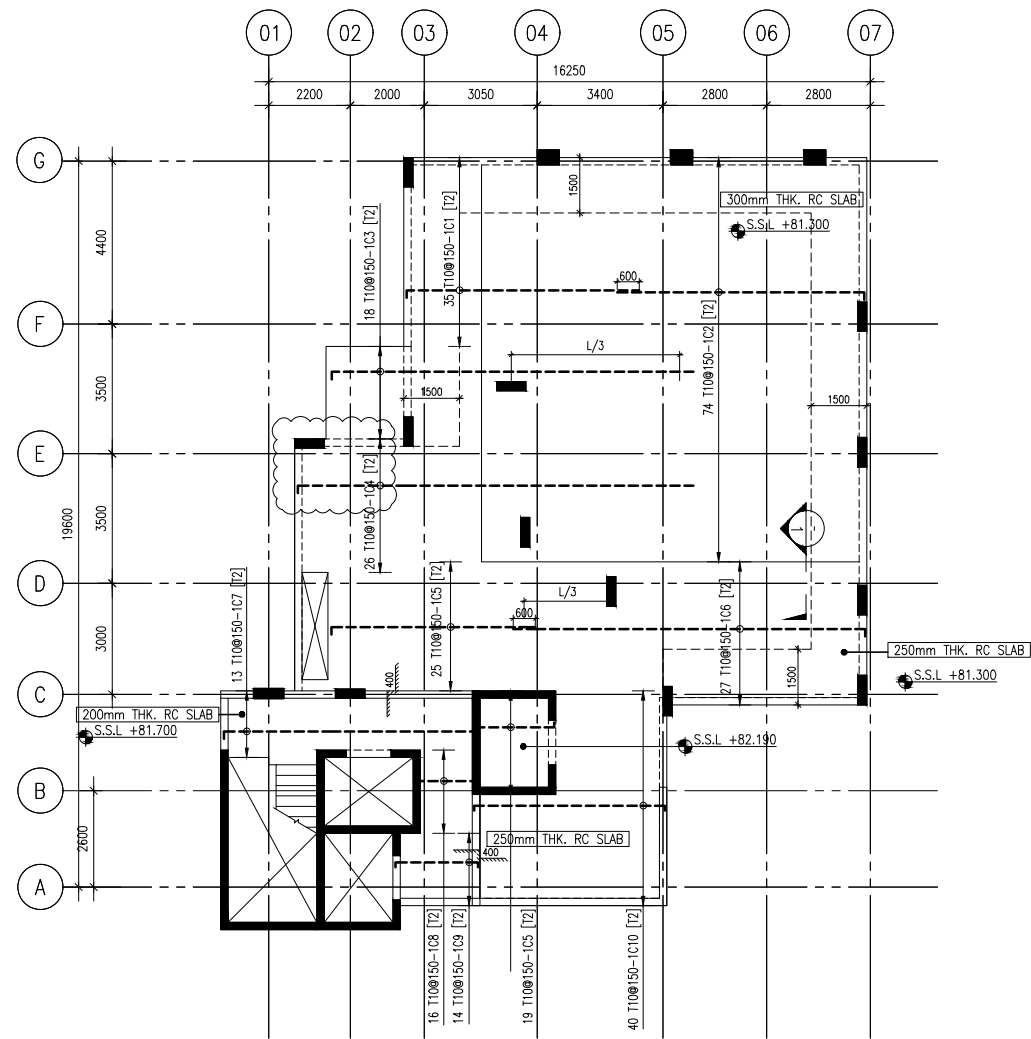
REINFORCEMENT DETAILS OF SLAB AT ROOF LEVEL TOP - T2 SCALE 1:100
