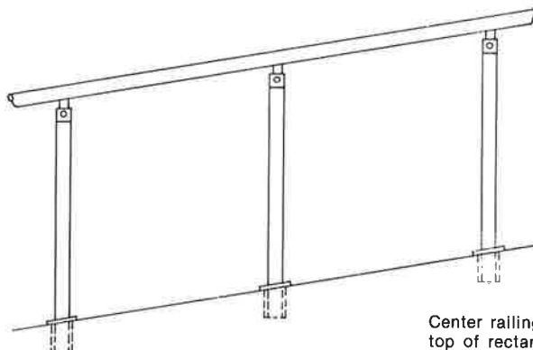
Fig. 81 Center railing of two members, with brackets to square or rectangular posts, steel, bronze or aluminum. Posts set into floor as at ends, or extended to subread and bolted as at center. Flanges loose or fixed.
