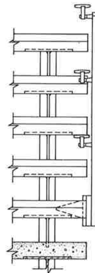
STRINGER INTERSECTION
