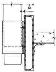
FIG. 66 Post mounted on box stringer.
