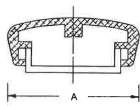
A = 2-3/4" Aluminum FIG. 91
