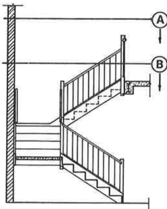
SECTION THROUGH STAIR
