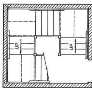
PLAN B
