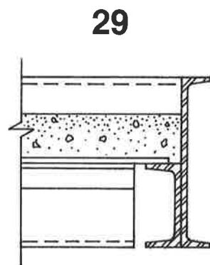
29 Edge of platform at open well. Face stringer attached to channel header. Channel stringer around platform.
