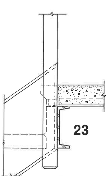
23 Stringers bolted or welded to channel header.
