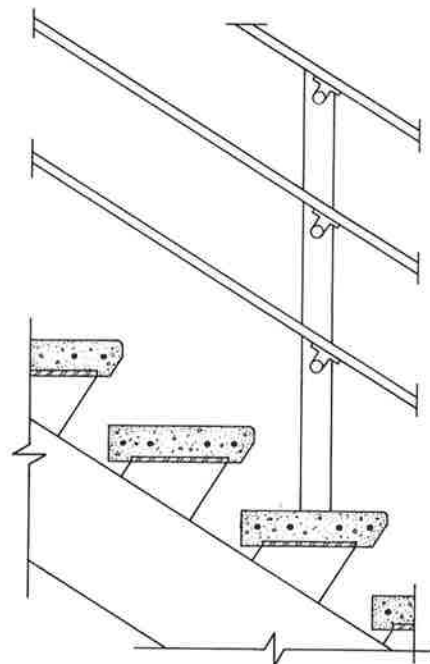
STRINGER INTERSECTION
