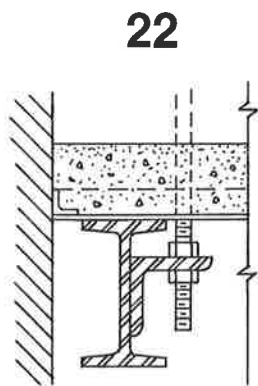
22 I-beam platform support suspended by hanger.
