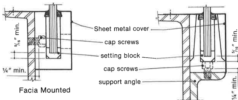
Facia Mounted
