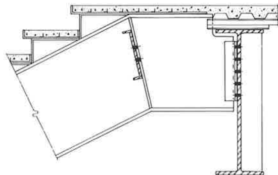
Stringer connection to existing steel
