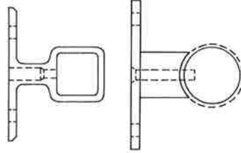
FIG. 65 Flanges for channel stringers.
