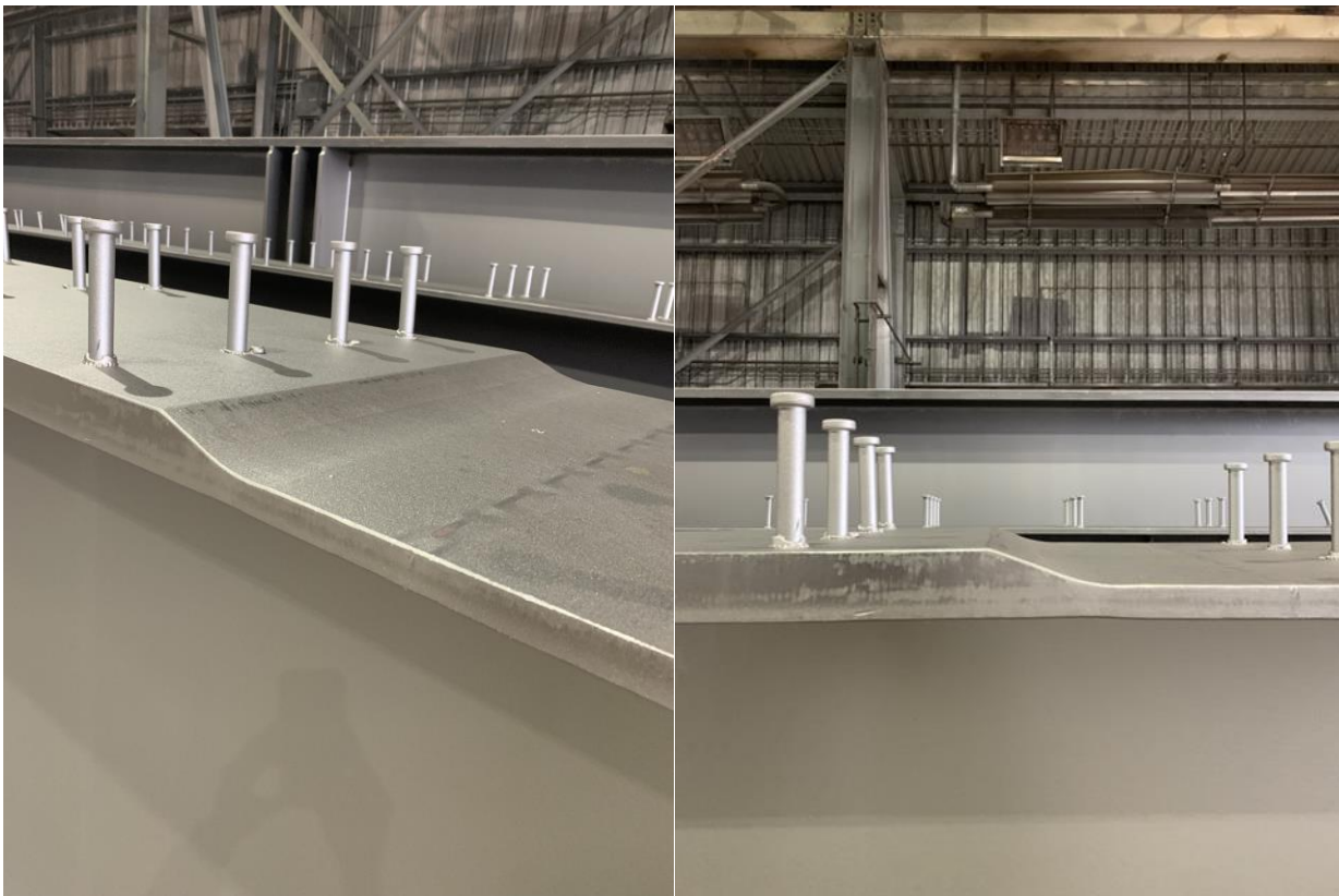
Figure 2.4.7-2—Where practical, flange thickness transitions are preferred for general constructability and corrosion performance.
