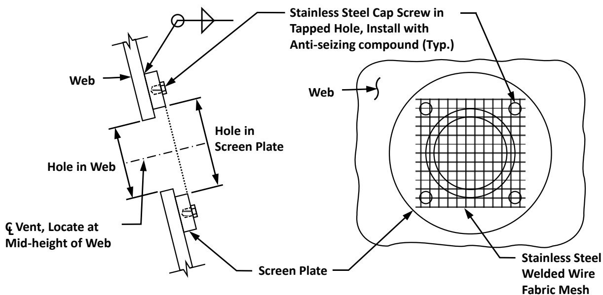
Figure 2.5.1-14—Example box girder screened vent hole detail.
