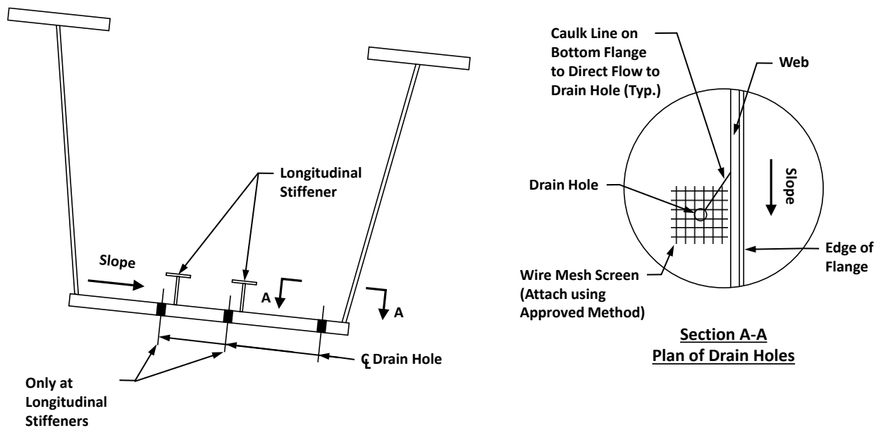
Figure 2.5.1-13—Example drain hole details
