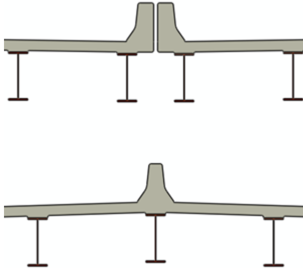
Figure 2.5.1-3—Example of eliminating closely spaced parallel structures or longitudinal joints.
