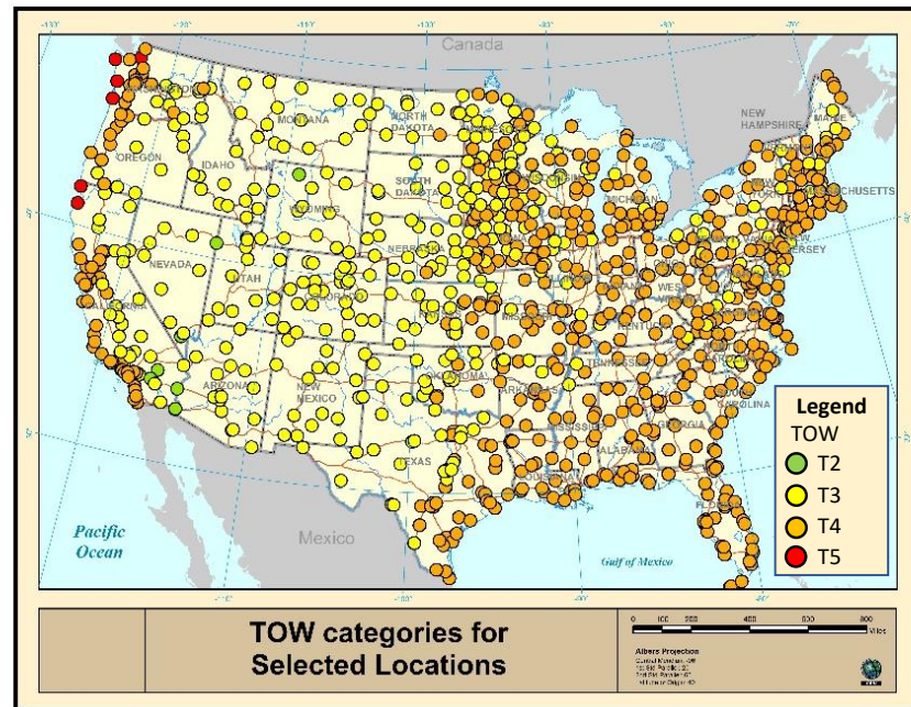
Figure 2.2.3.1-1—Time of Wetness Categories for Selected Locations in U.S.
