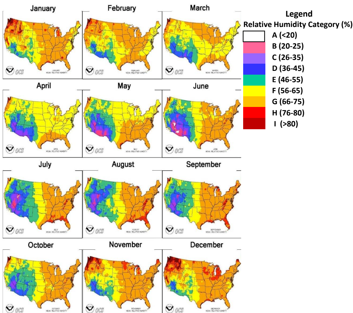
Figure 2.2.3.2-1—Monthly Relative Humidity Averages in the U.S.
