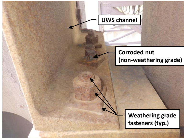
Figure 2.5.4.6.1-1—Corrosion of non-weathering grade nut.
