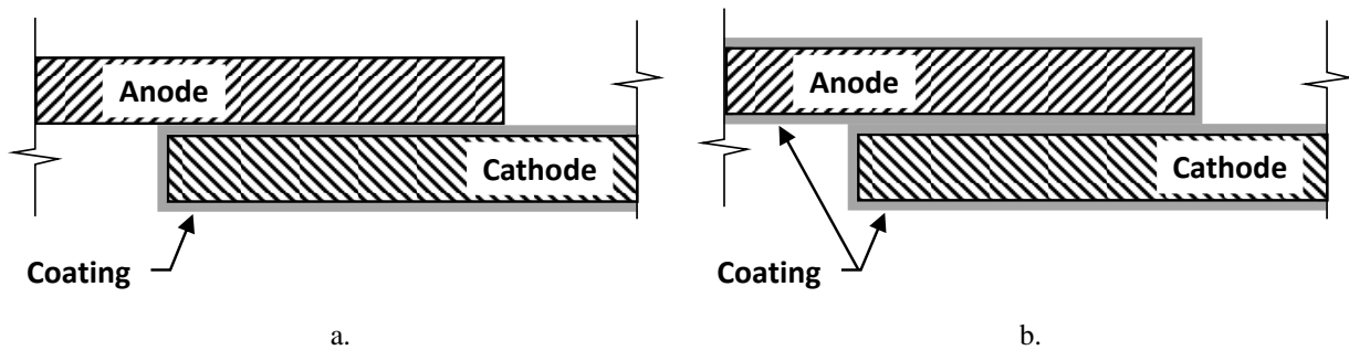
Figure 2.5.4.5-2—Coating methods to prevent galvanic corrosion (a) coat the cathode (b) coat both the cathode and anode.
