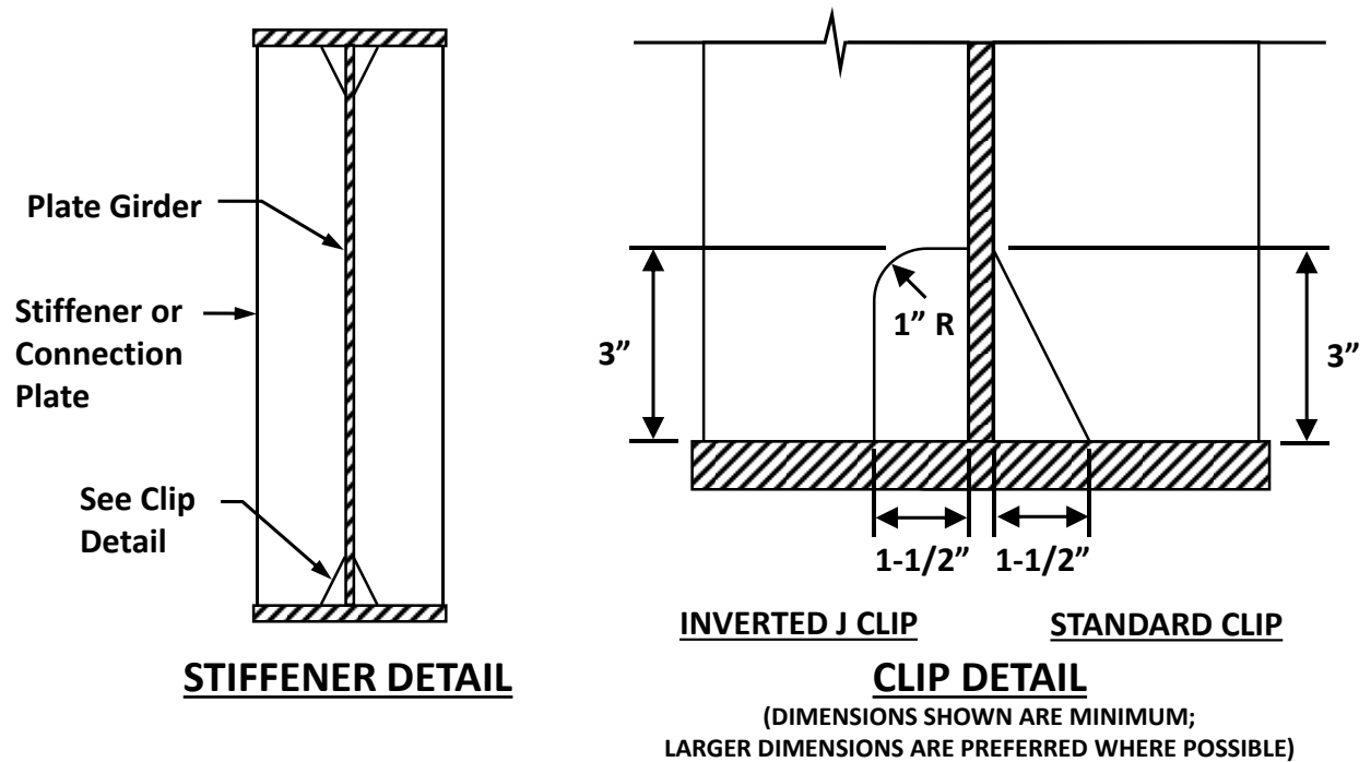
Figure 2.5.2-1—Size stiffener clips to avoid trapping debris.
