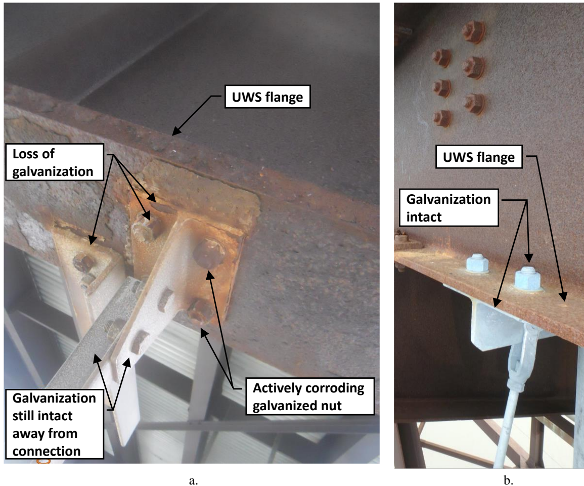
Figure 2.5.4.6.3-1—Example of dissimilar metal appurtenance attachments to UWS: (a) galvanically corroding galvanized attachment (b) non-corroded galvanized attachment.
