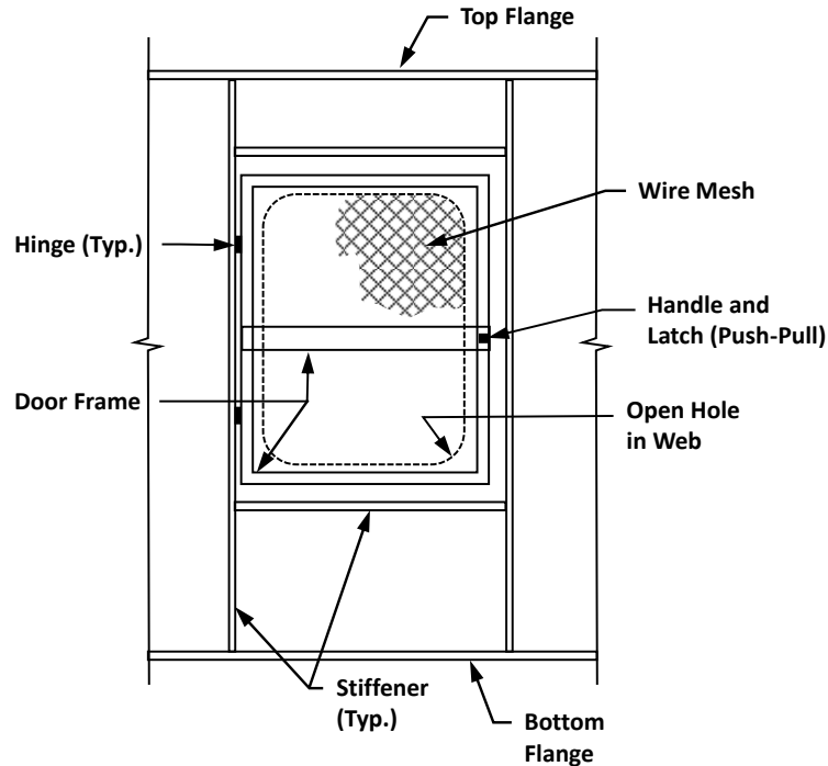
Figure 2.4.1.2-1—Example Vented Access Door.
