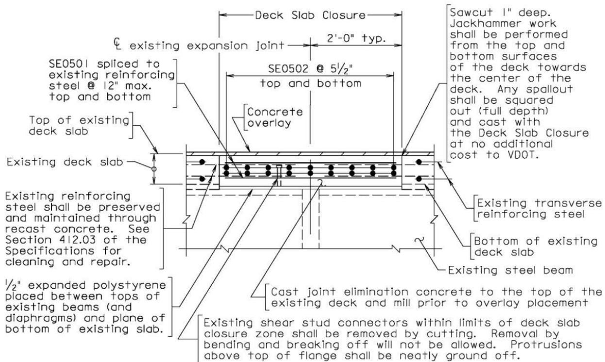
Figure 6.1.4-1—Link slab construction on existing bridge.
