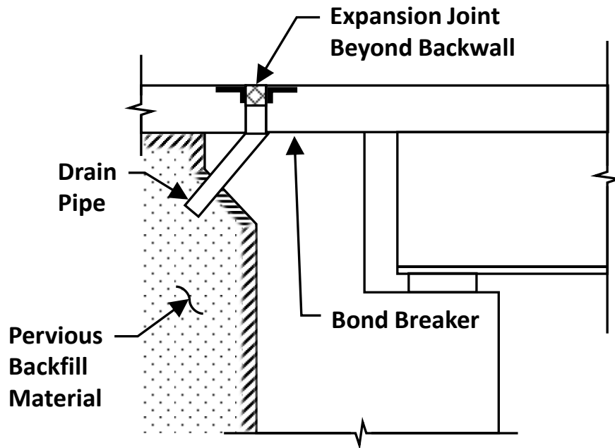
Figure 2.5.1-10—Example of locating the expansion joint at the back of the backwall.
