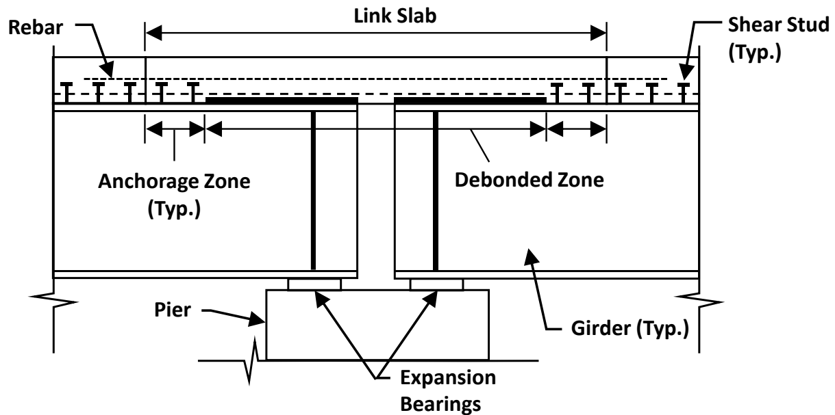
Figure 2.5.1-2—Example of a link slab to eliminate a joint at intermediate supports for simple span designed bridges. Expansion and contraction from thermal movements to abutment ends.
