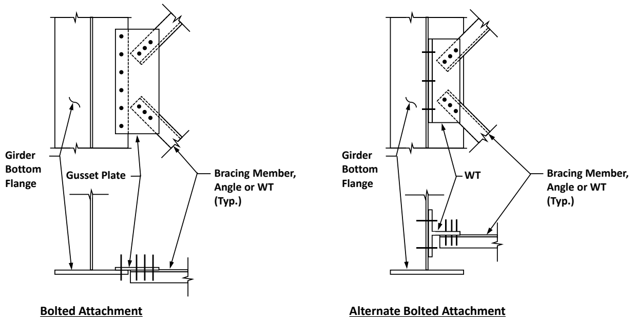
Figure 2.5.2-4—Preferred lateral bracing connection details.
