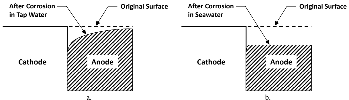
Figure 2.5.4.4-1—Effect of electrolyte resistivity on galvanic corrosion: (a) in tap water (high resistance) (b) in seawater (low resistance).
