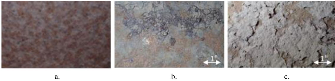
Figure 4.1.1.2-3—Photographs of poor performance of UWS showing various textures: (a) rough "freckled" surface, (b) a relatively smooth surface that was easily crushed by tapping, (c) coarse surface with exfoliating rust layers.
