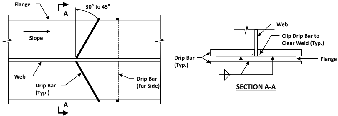
Figure 2.5.1-5—Example drip bar detail.
