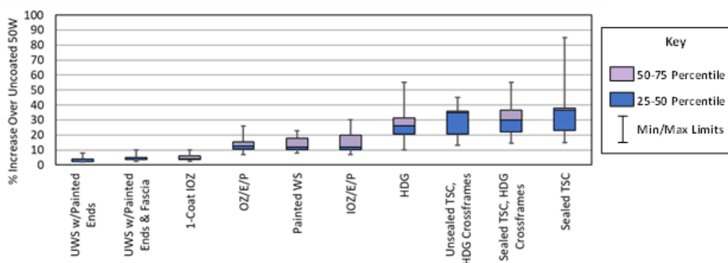
Figure 1.1.1-2—UWS provides the minimal first cost (shown here using box and whisker plot of 2020 data) and life-cycle cost for typical girder bridges.
