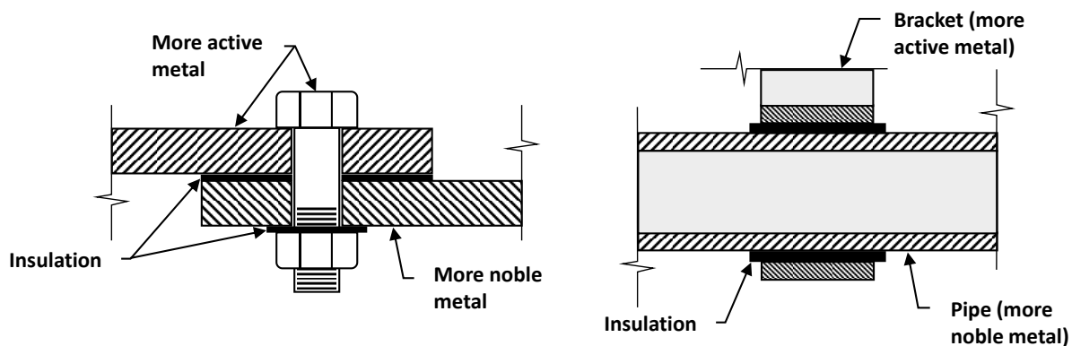
Figure 2.5.4.5-1—Insulation methods to prevent galvanic corrosion.
