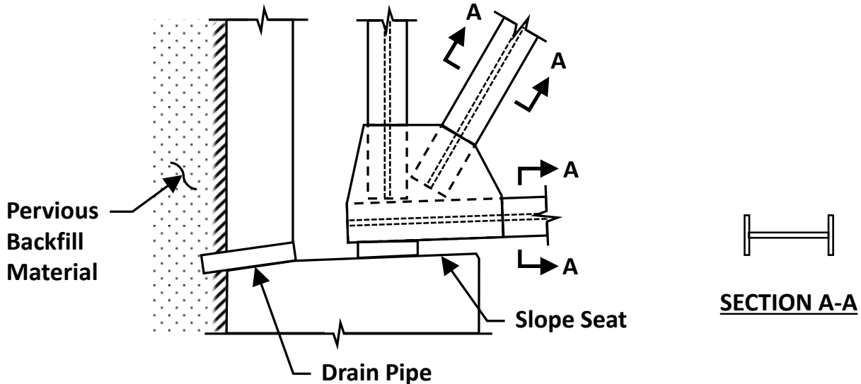
Figure 2.5.1-11—Example of sloping abutment seat and truss orientation for drainage.
