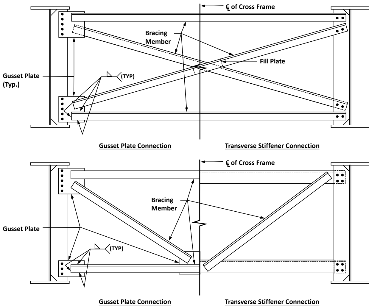
Figure 2.5.2-2—Preferred cross frame details.
