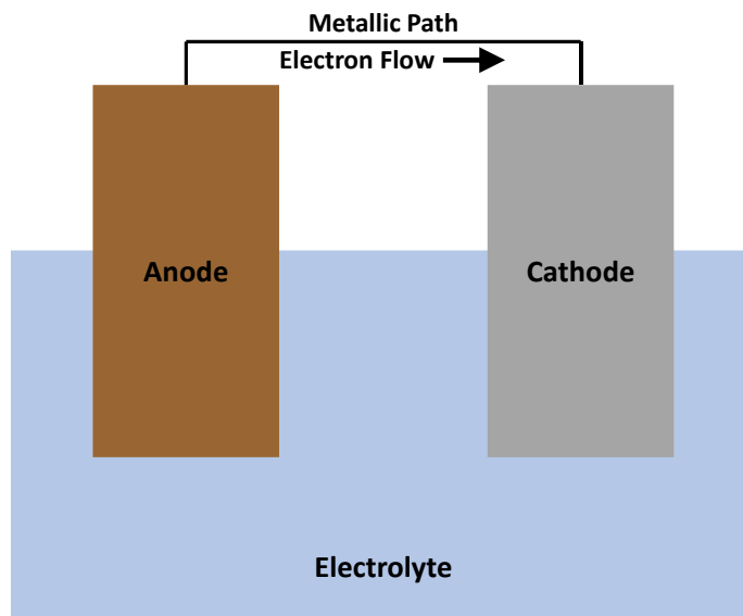
Figure 2.5.4.1-1—Galvanic corrosion mechanism.
