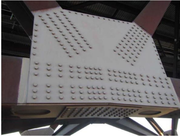
Figure 6.1.1-2—Painted weathering steel bolted connections (a) truss gusset plate (b) girder splice.
