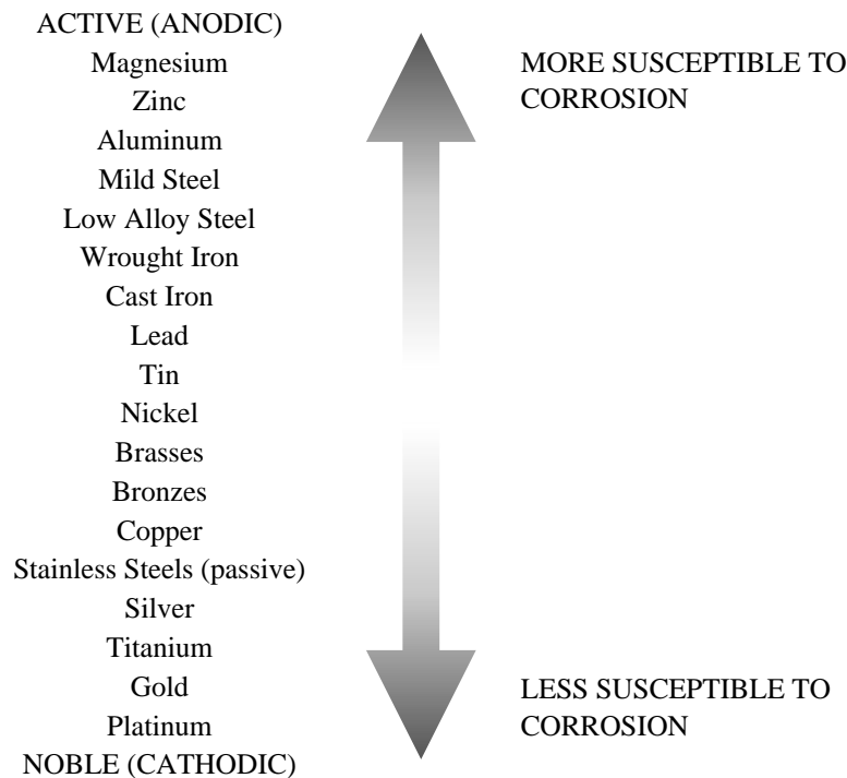
Figure 2.5.4.2-1—Galvanic Series of Metals in Seawater.
