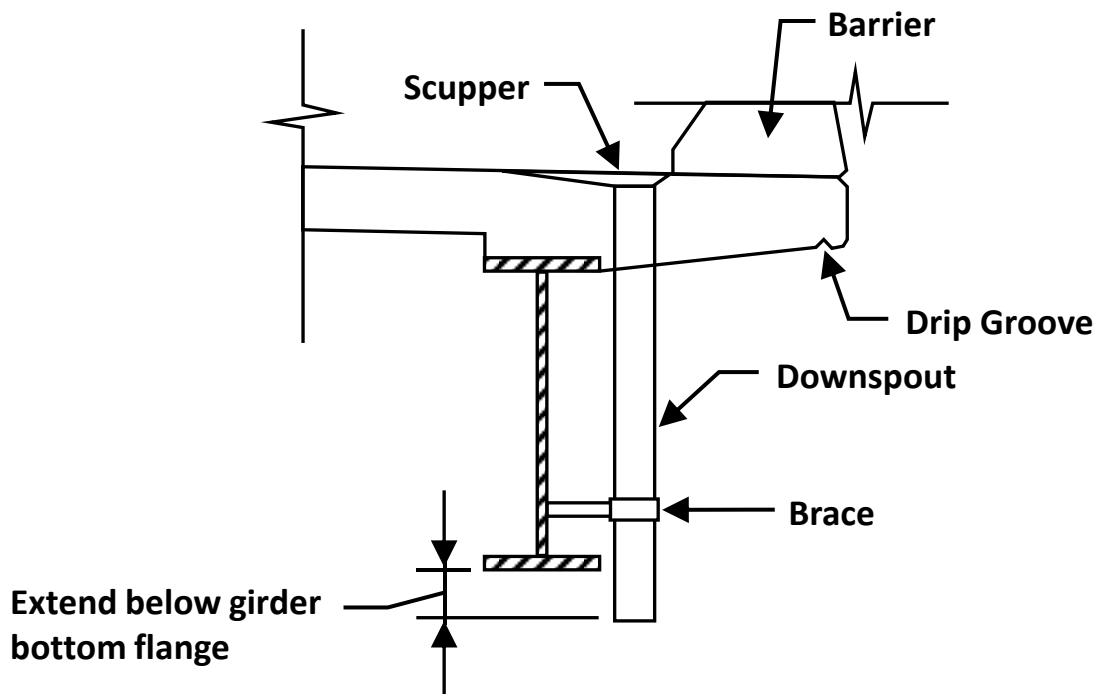
Figure 2.5.1-8—Example downspout detail.
