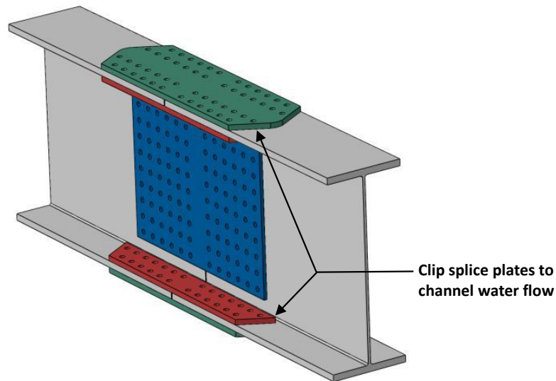
Figure 2.5.2-3—Illustration of clipping splice plates.
