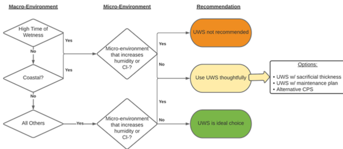
Figure 2.1-1—General Concept for UWS use Based on Macro- and Micro-Environment
