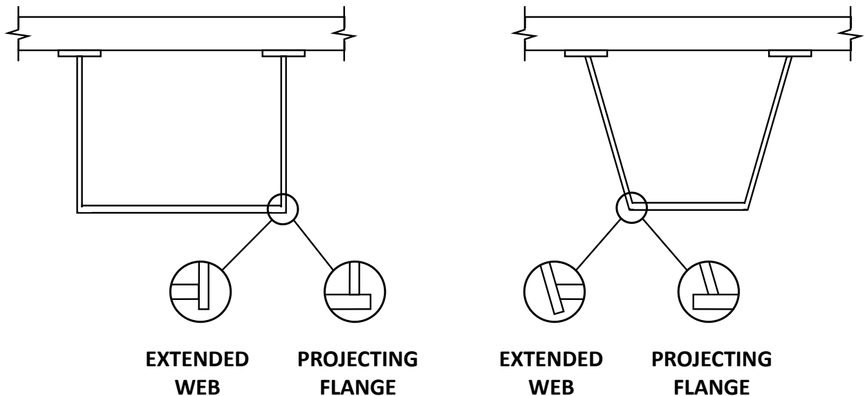
Figure 2.5.1-12—Example box girder fabrication details.
