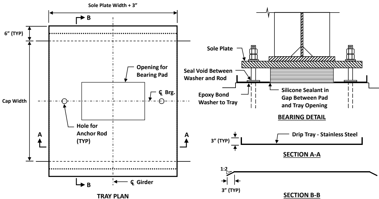
Figure 2.5.1-7—Example drip tray detail.
