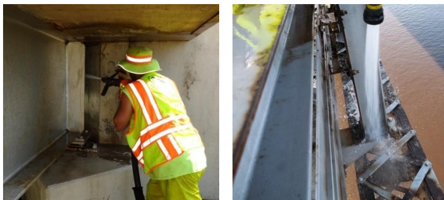
Figure 5.1.3.2.1-1—Deck component cleaning (a) roadway and parapet (b) expansion joint (c) drainage components.
