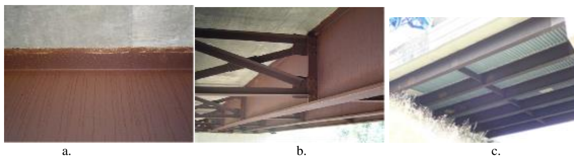
Figure 4.1.1.2-4—Photographs showing typical color progression of good-performing UWS in U.S. environments: (a) relatively new bridge (less than 10 years), (b) bridge in early stages of service life (less than 25 years), (c) bridge with advanced patina development. Note: Color, perception of color, and rate of color change can be highly variable and dependent on environment, lighting conditions, etc.
