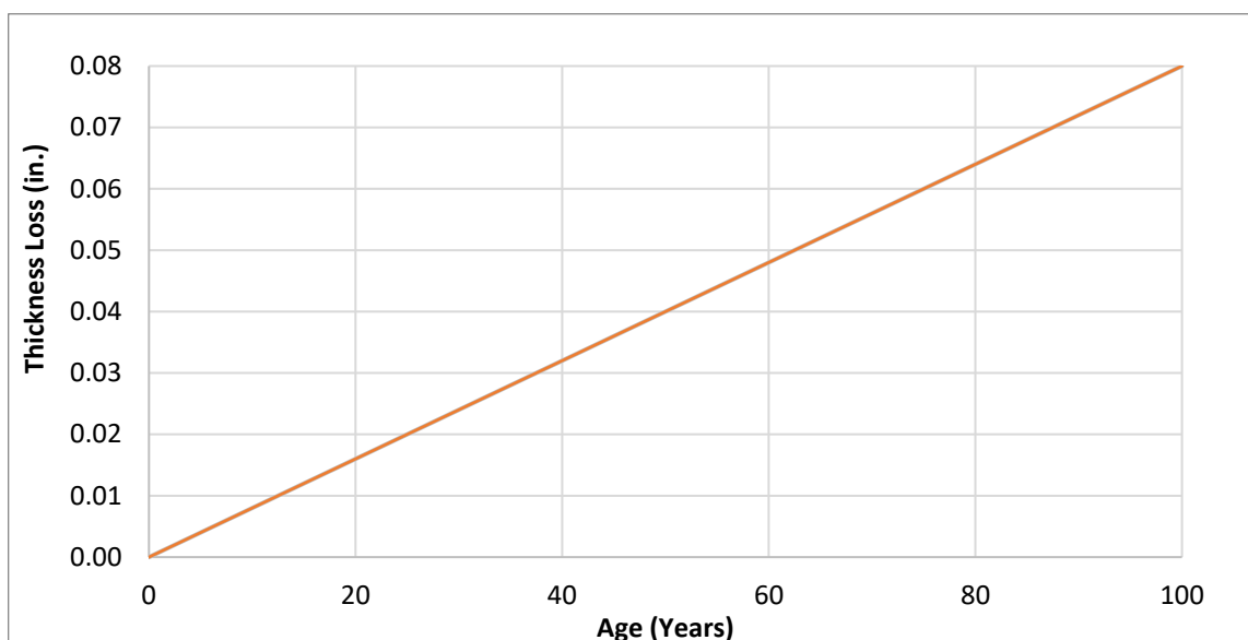
Figure 2.4.3-1—Estimated upper-bound section loss for fully-exposed UWS plates (i.e., total section loss on top and bottom surfaces) in "high" corrosive environments.
