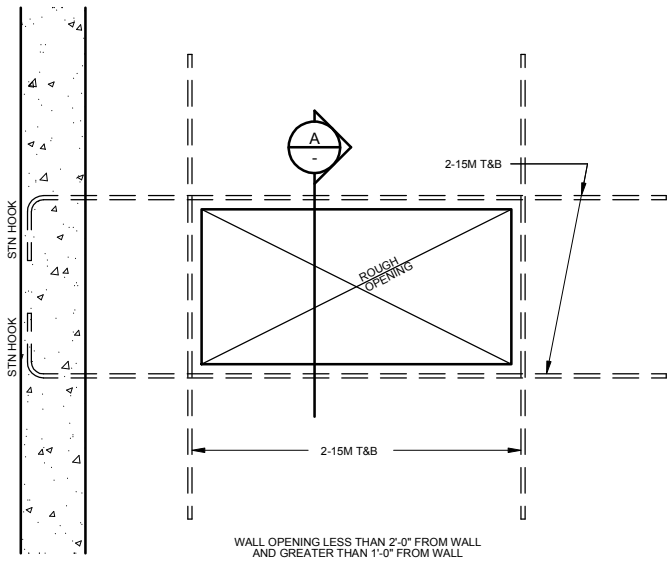
TYPICAL WALL OPENINGS SCALE: NTS RFG SHOWN IS IN ADDITION TO WALL RFG
