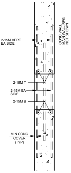
B SECTION NTS
