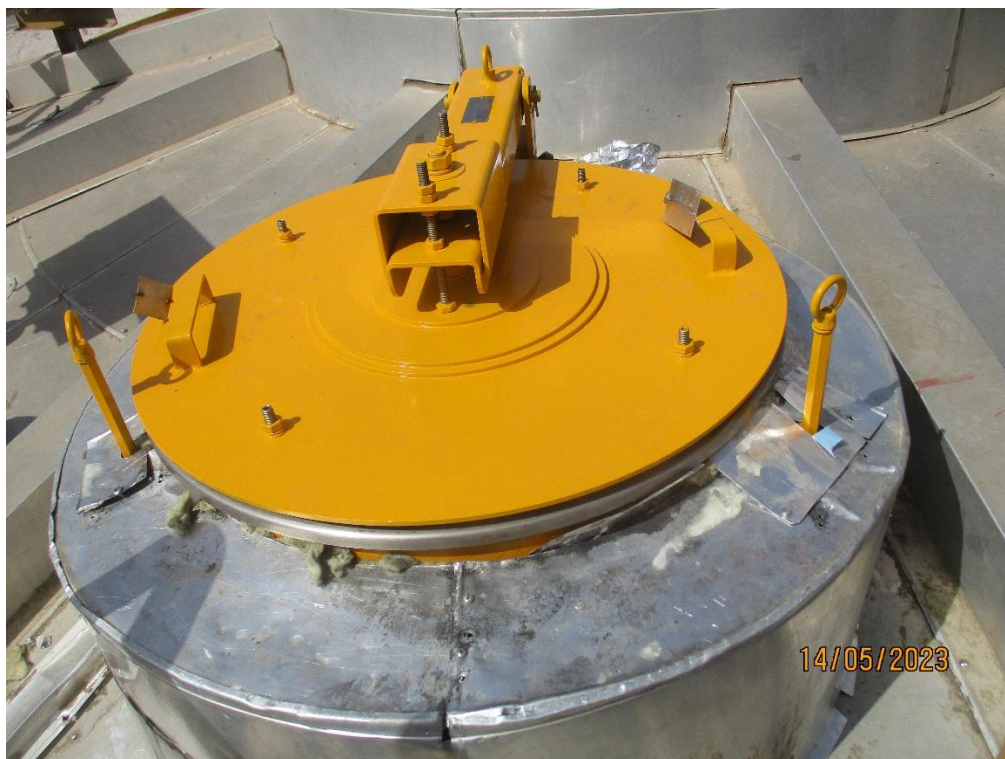
901 -ERV-027 Electrical heat tracing
