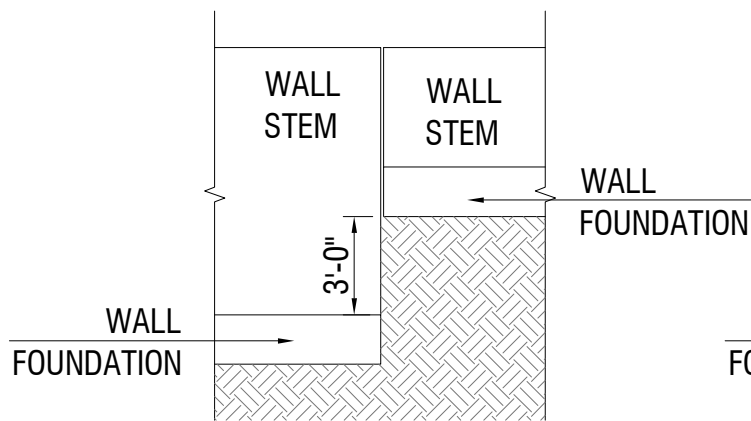
ELEVATION OF RETAINING WALL
