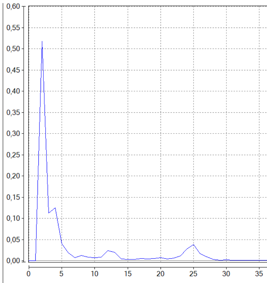
Velocity spectrum on motor base when pump unit is not working
