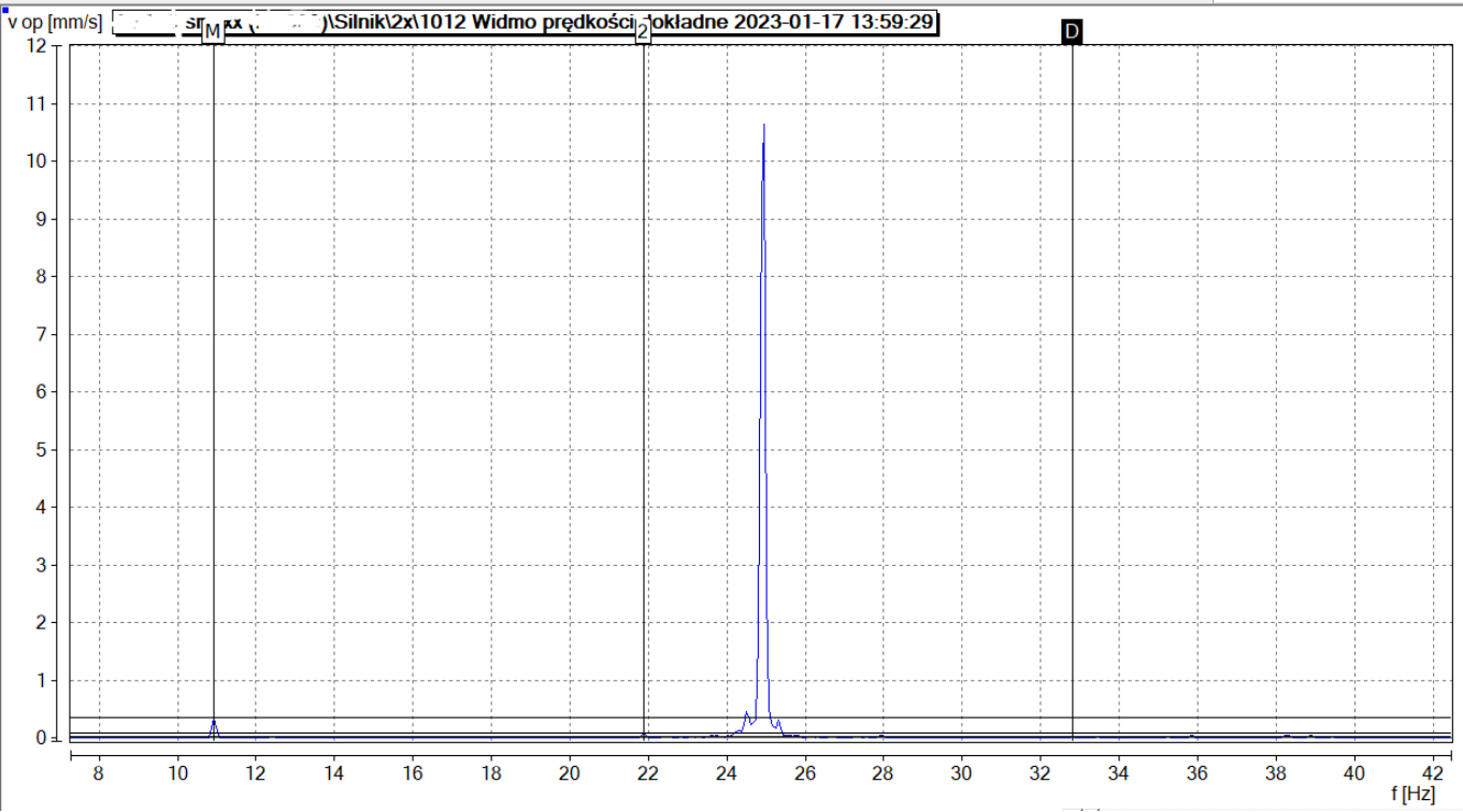
High frequency velocity spectrum @ 656 rpm:
