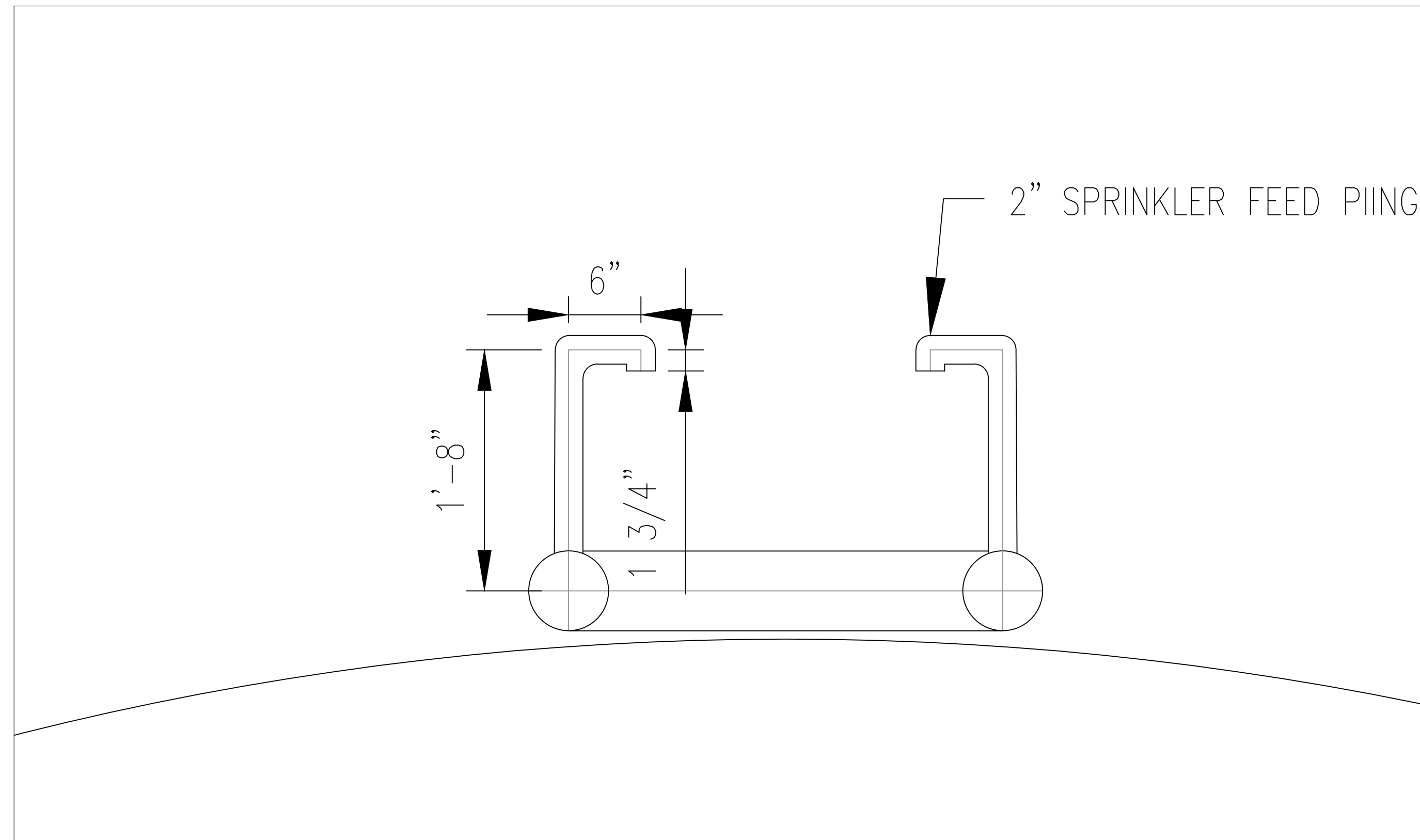
SECTION B 1/2"=1'-0"
