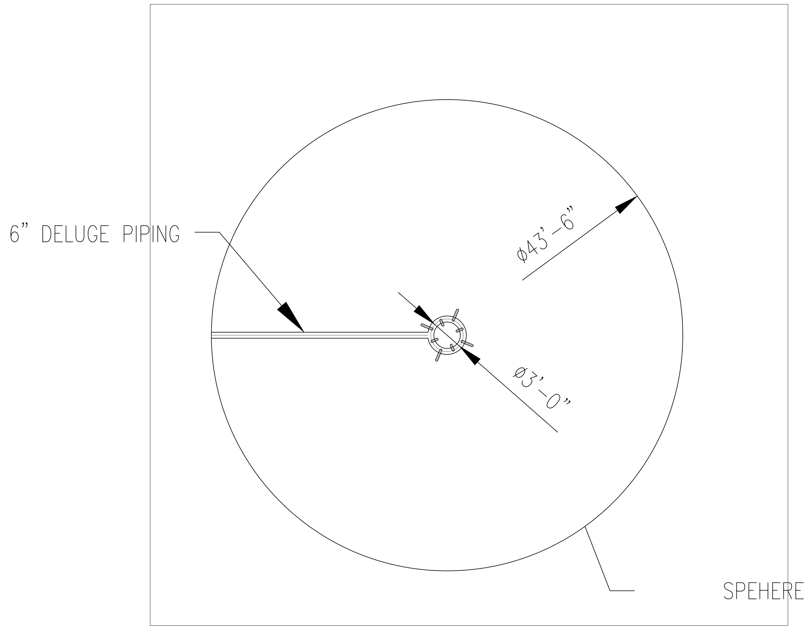
PLAN VIEW 1/16"=1'-0"
