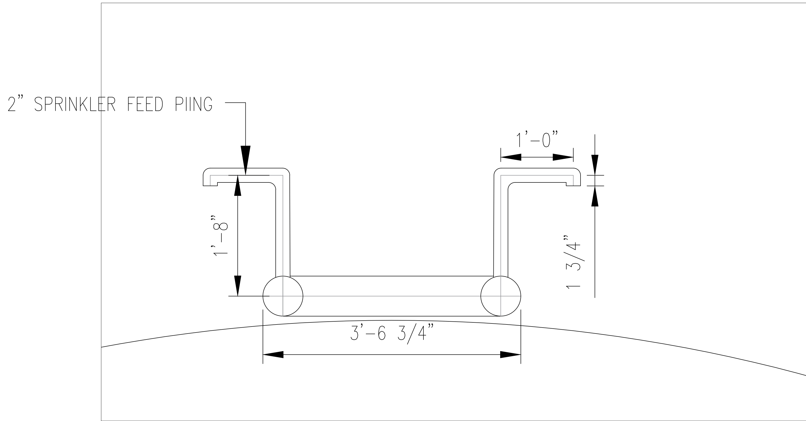
SECTION A 1/2"=1'-0"
