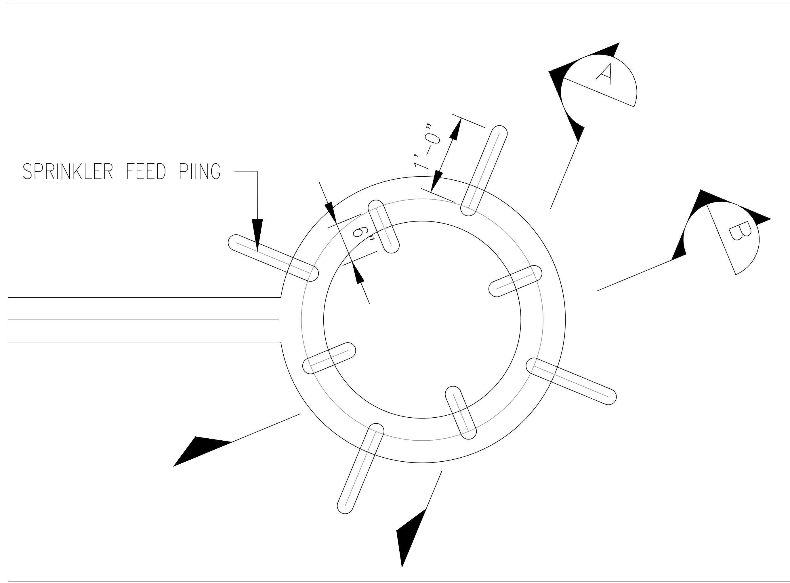
PLAN VIEW 1/2"=1'-0"
