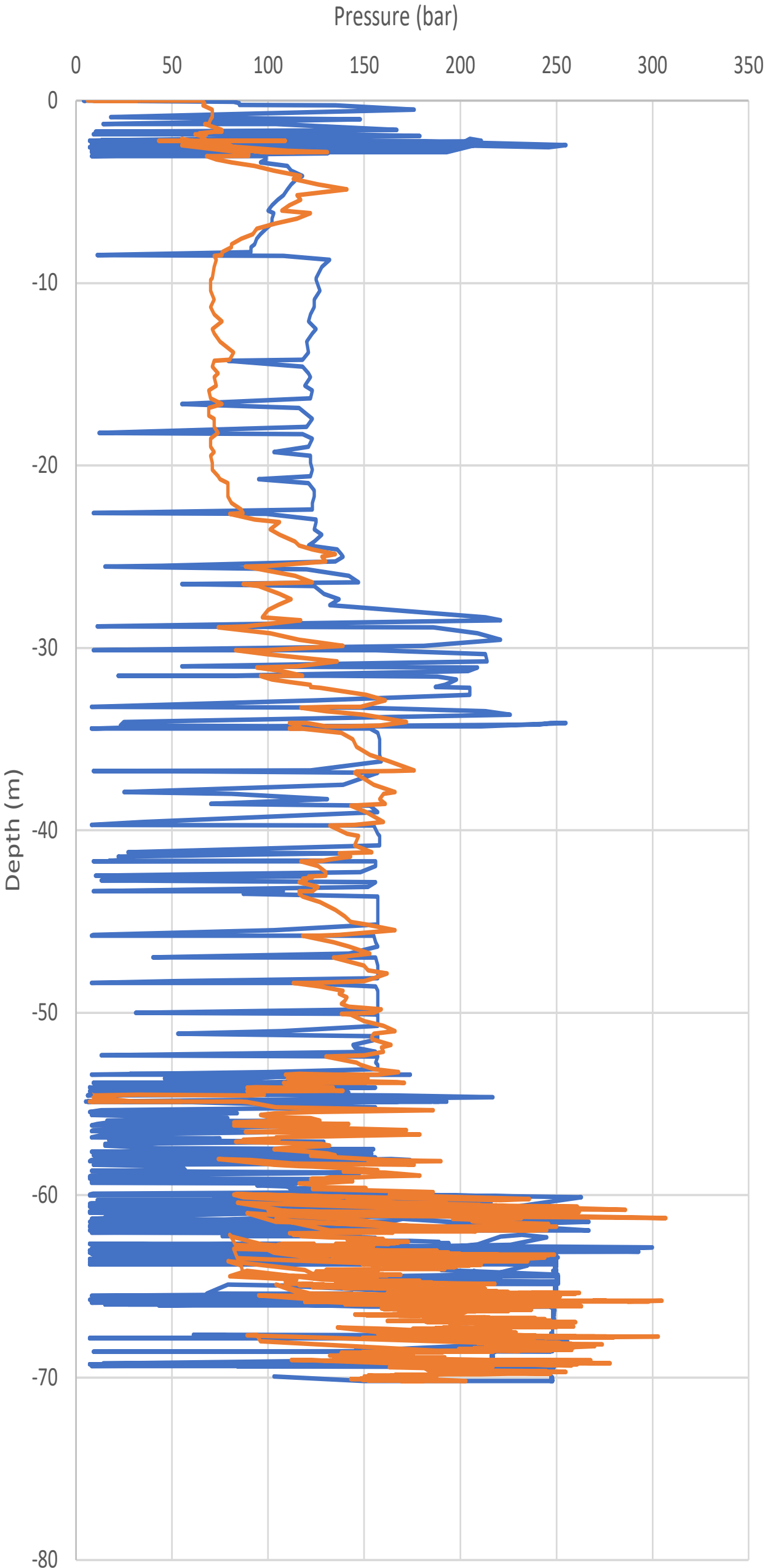
TEST PILE INSTALLATION DATA FROM DRILL RIG
