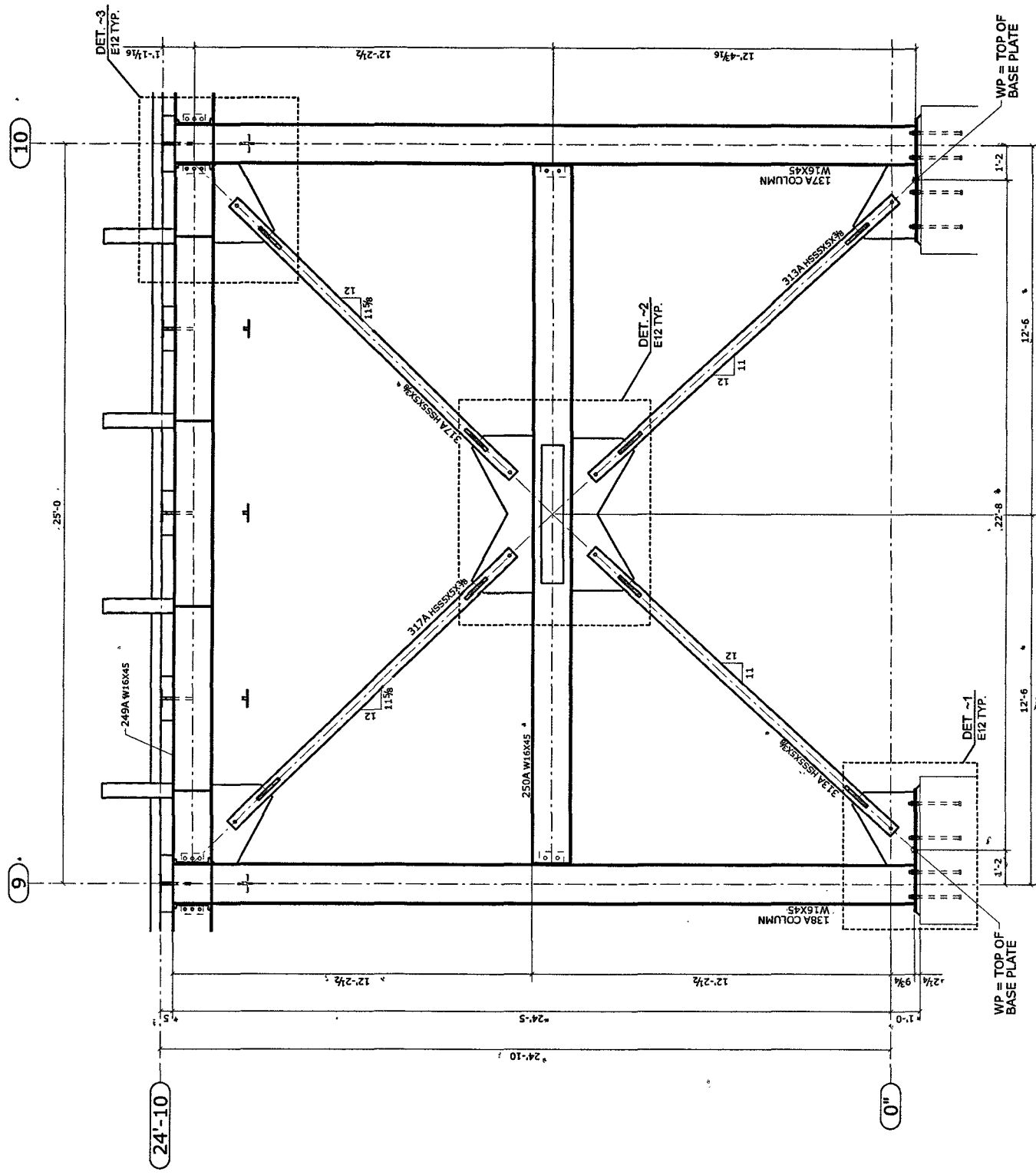
PARTIAL ELEVATION VIEW ALONG GRID C
