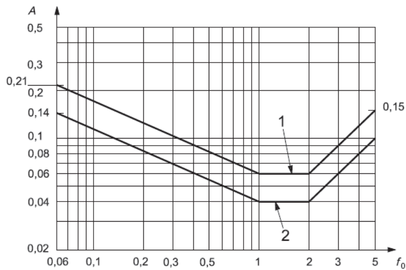
Figure 2.5: Acceptable accelerations according to ISO 10137:2008 [21].
