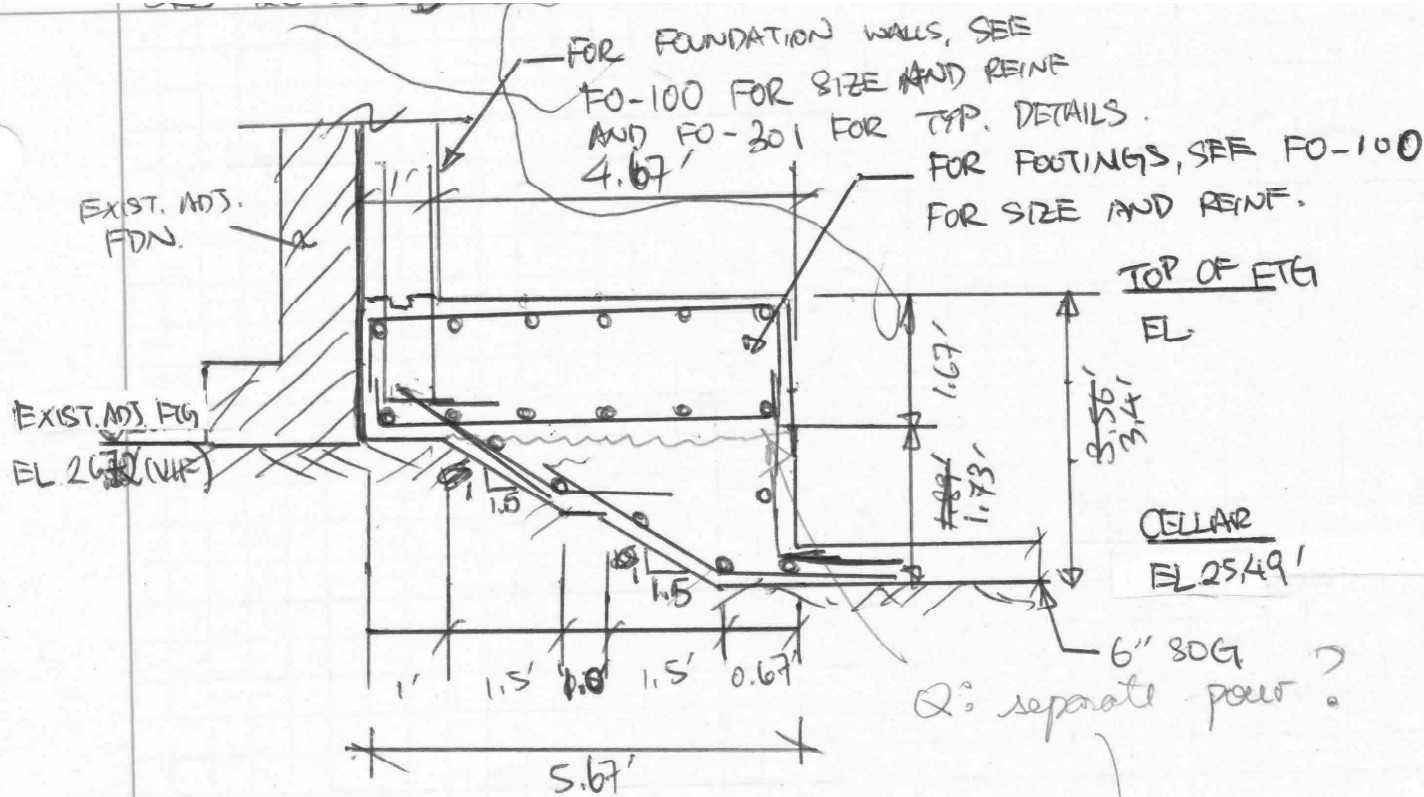
SECT B. NTS
