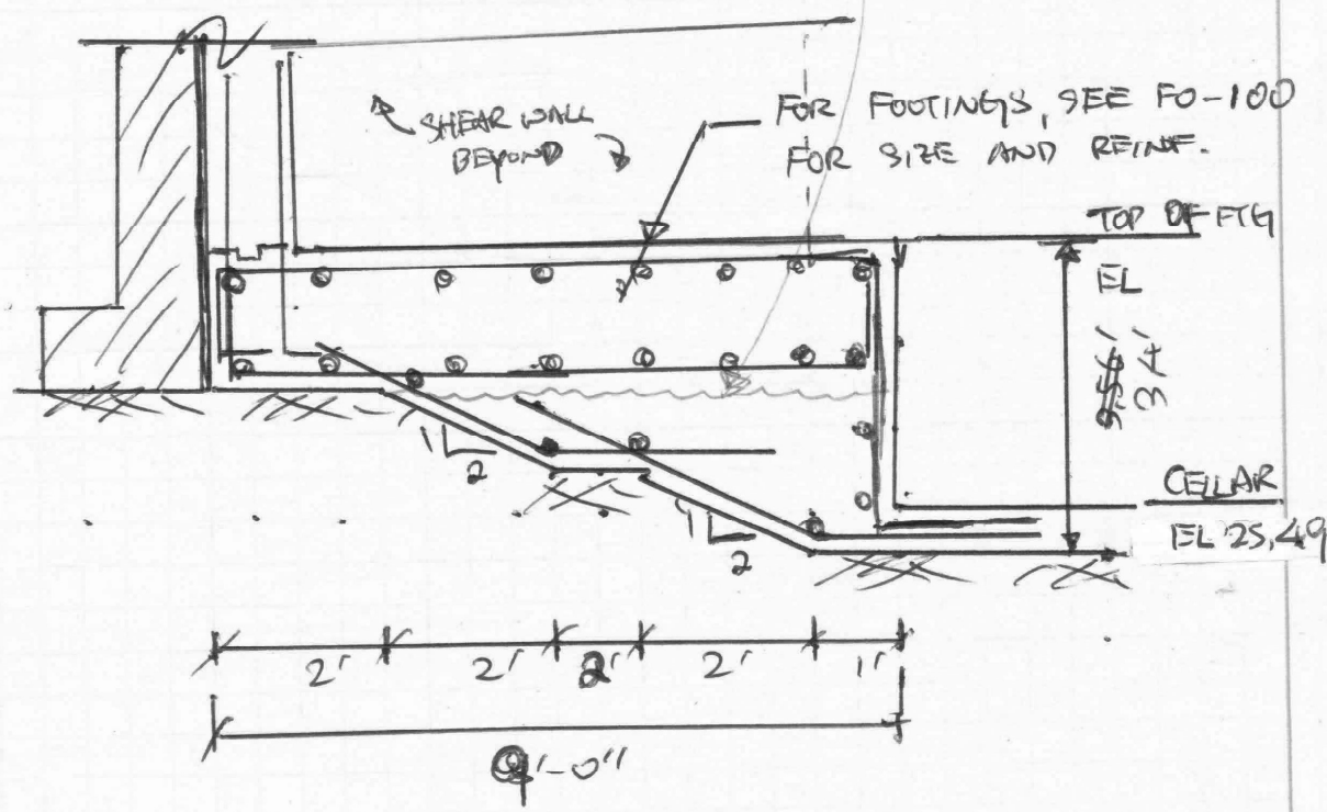
SECT C NTS
