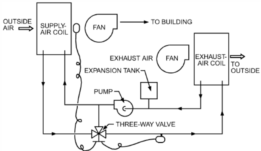
Fig. 8 Coil Energy Recovery Loop
