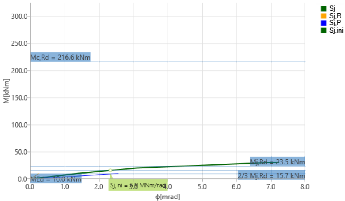
Stiffness diagram M_z - \phi_z , LE1
