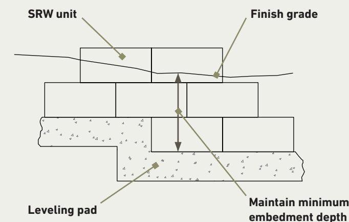
Figure 5.8-1 | Wall Step-Ups
