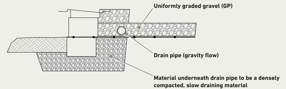
Figure 4.1.2-7 | Alternate Drain Pipe Location with Blanket Drain
