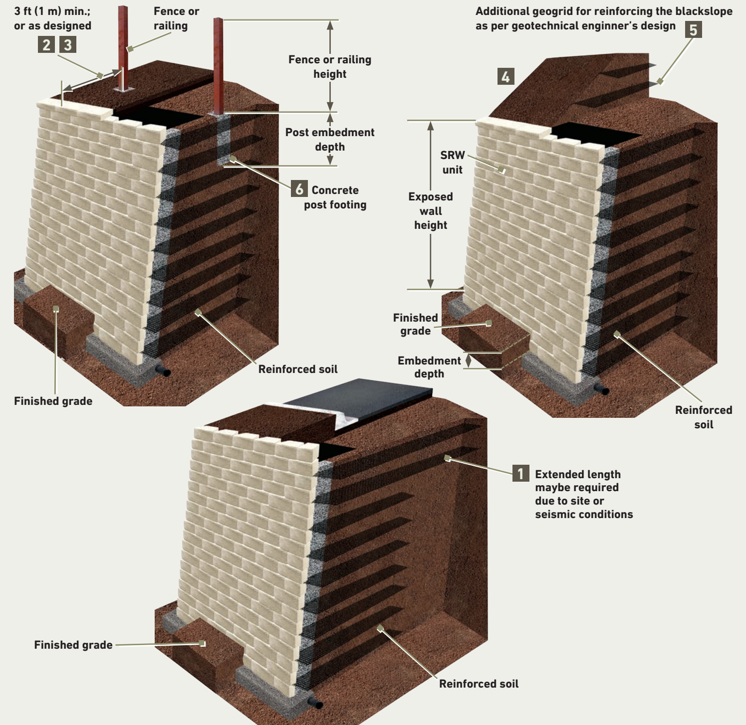
Figure 13 | Above Wall Considerations
