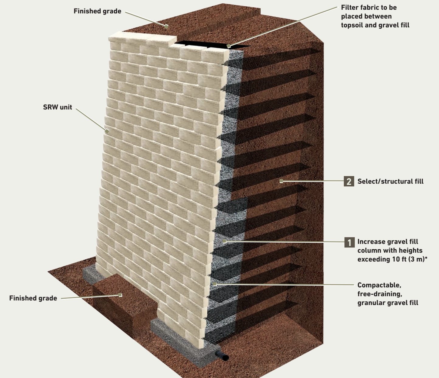
Figure 8 | Tall Walls
