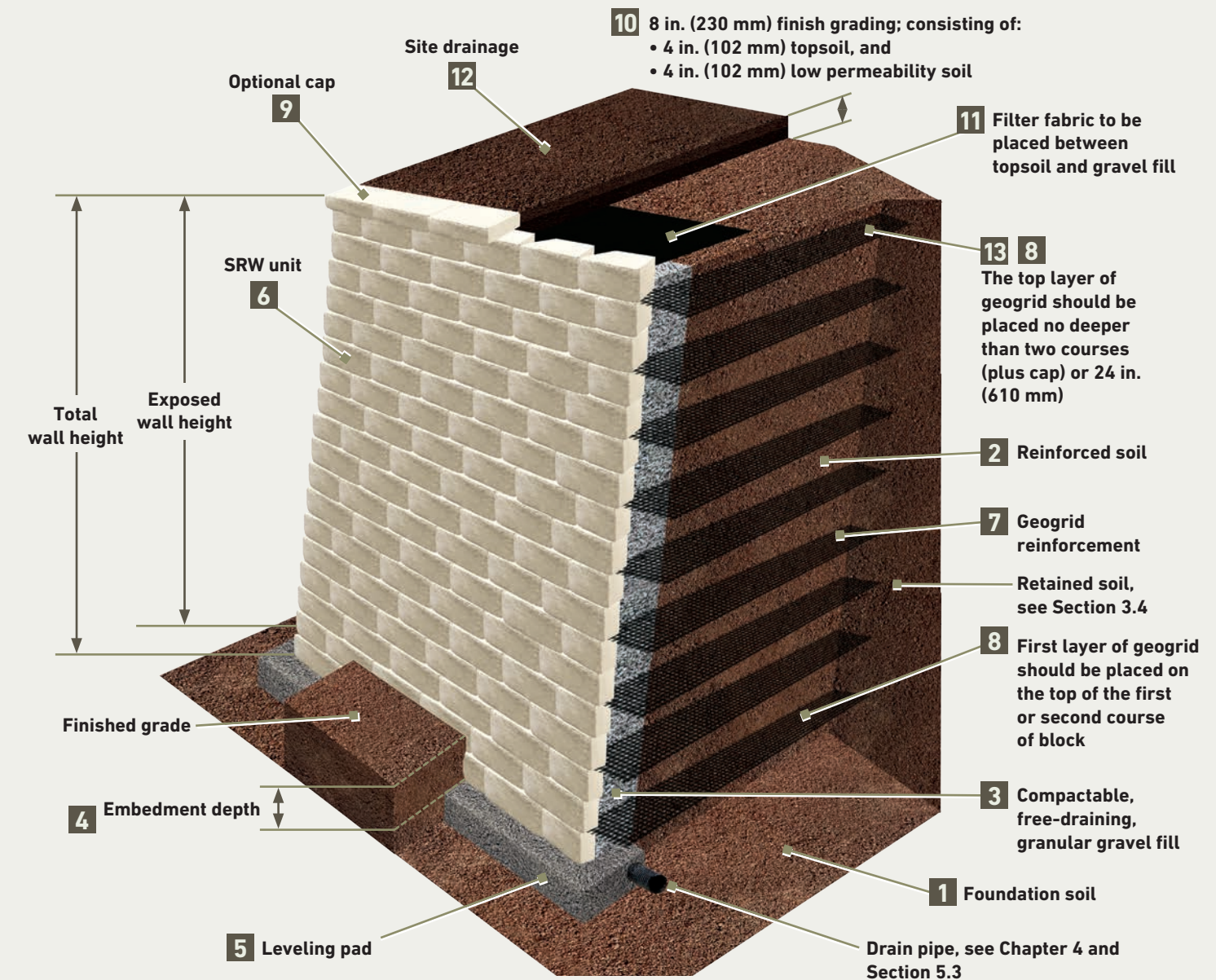
Figure 1 | General Criteria
