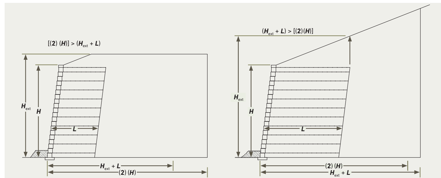
Figure 1.2-1 | SRW Design Envelope Limits
