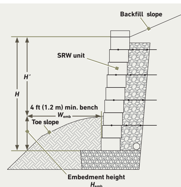
Figure 1.3-1 | Minimum Wall Embedment Depth, H_{emb}
