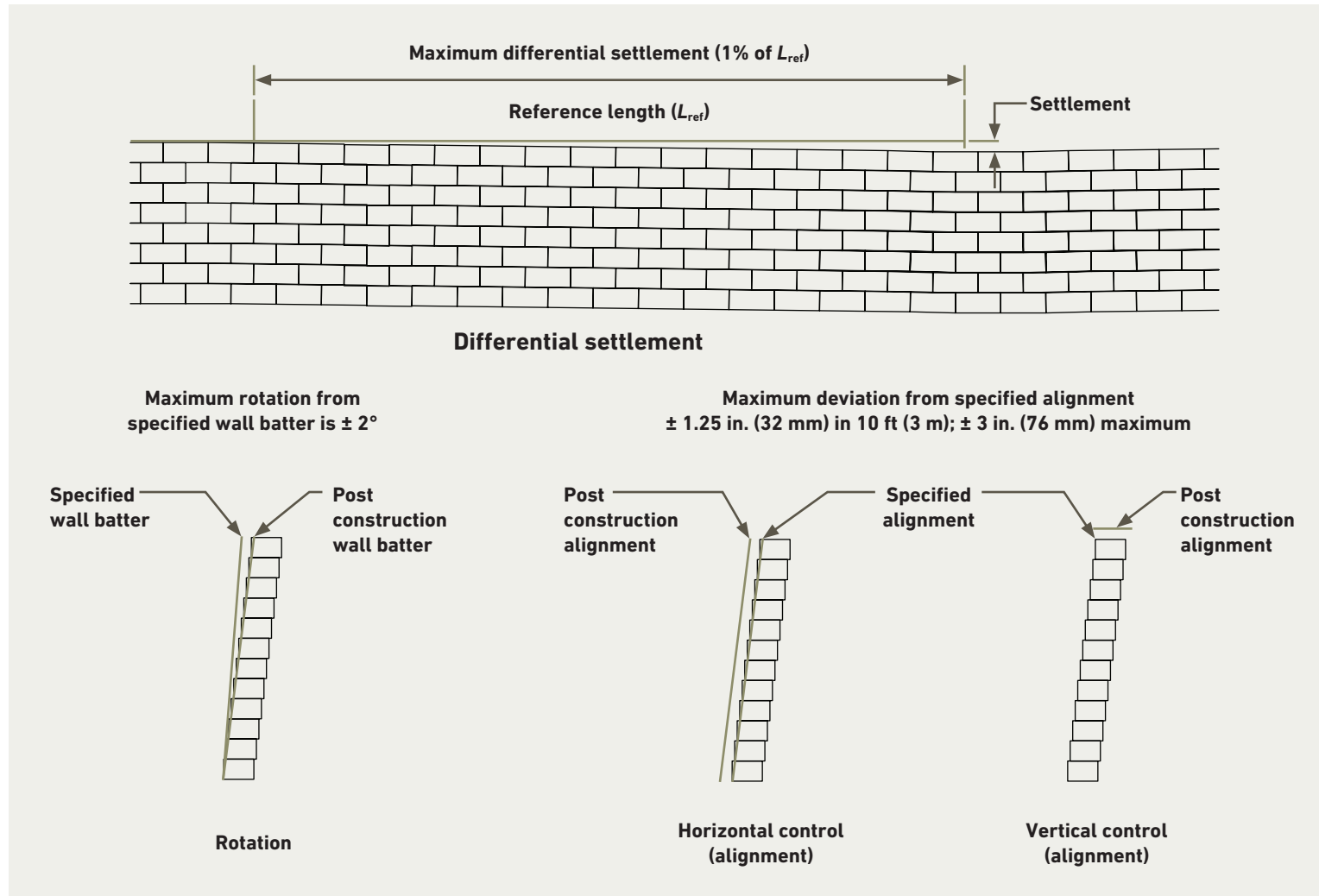
Figure 5.10-1 | Recommended SRW Construction Tolerances
