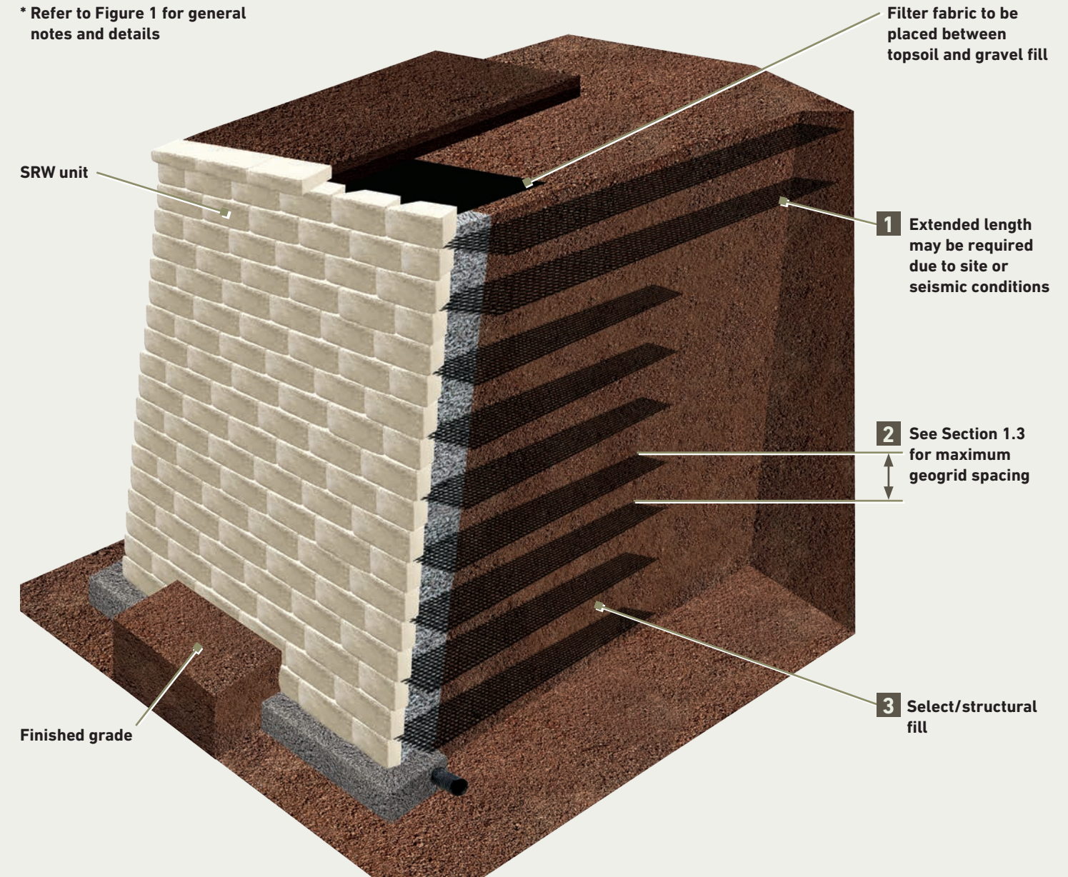
Figure 12 | Seismic Considerations
