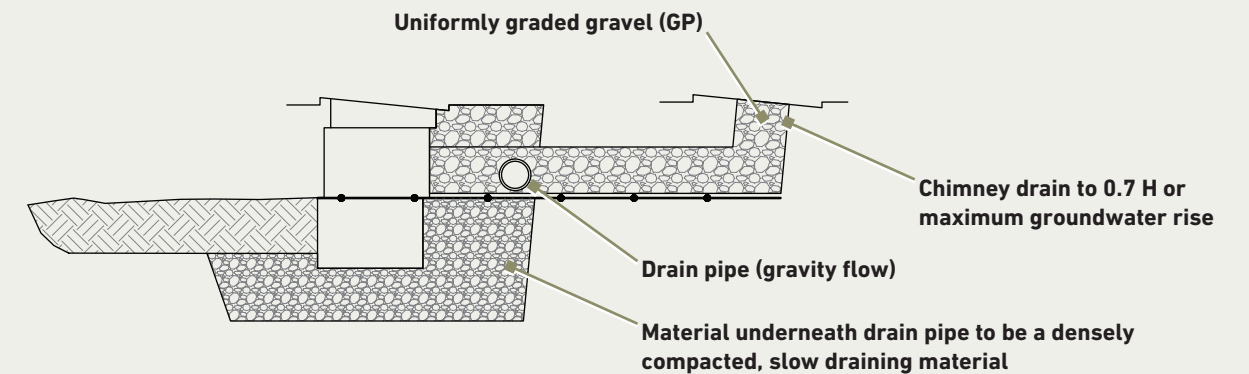
Figure 4.1.2-8 | Alternate Drain Pipe Location with Blanket Drain and Chimney Drain
