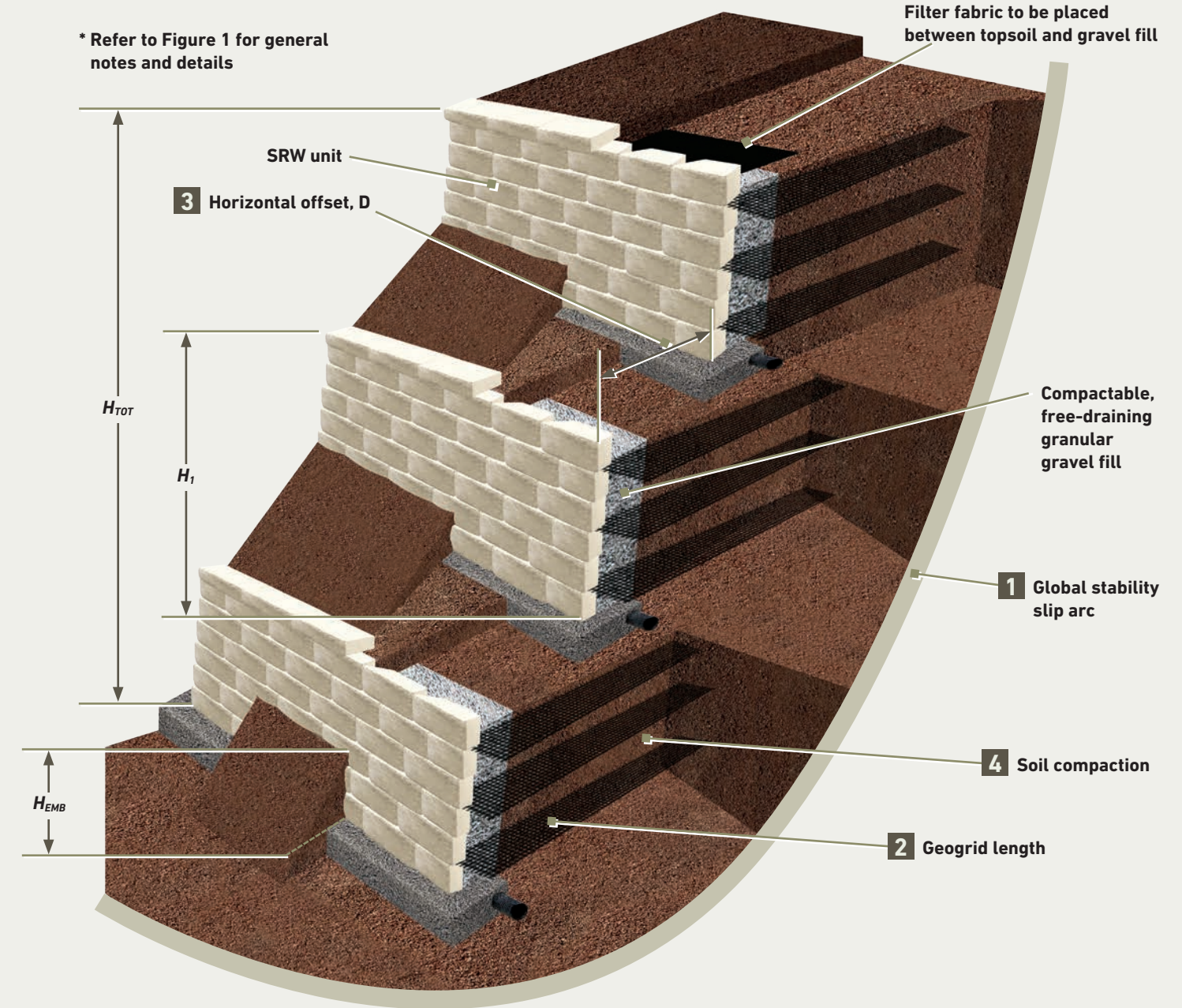
Figure 10 | Terraced Walls
