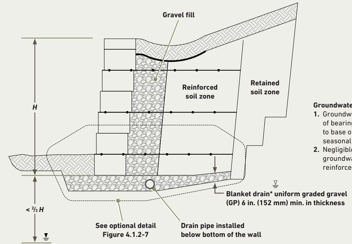
Figure 4.1.2-5 | Blanket Drainage System
