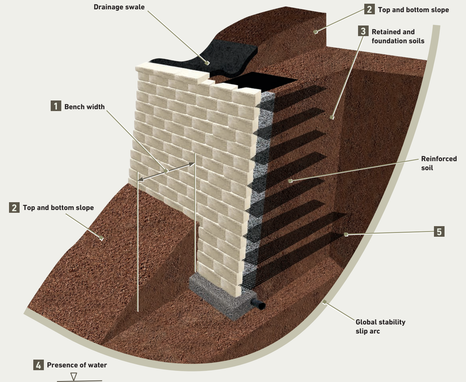
Figure 9 | Global Stability
