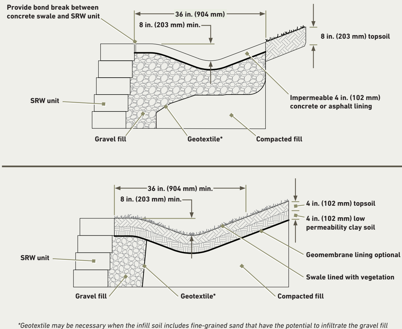
Figure 4.1.1-1 | Drainage Swale Details
