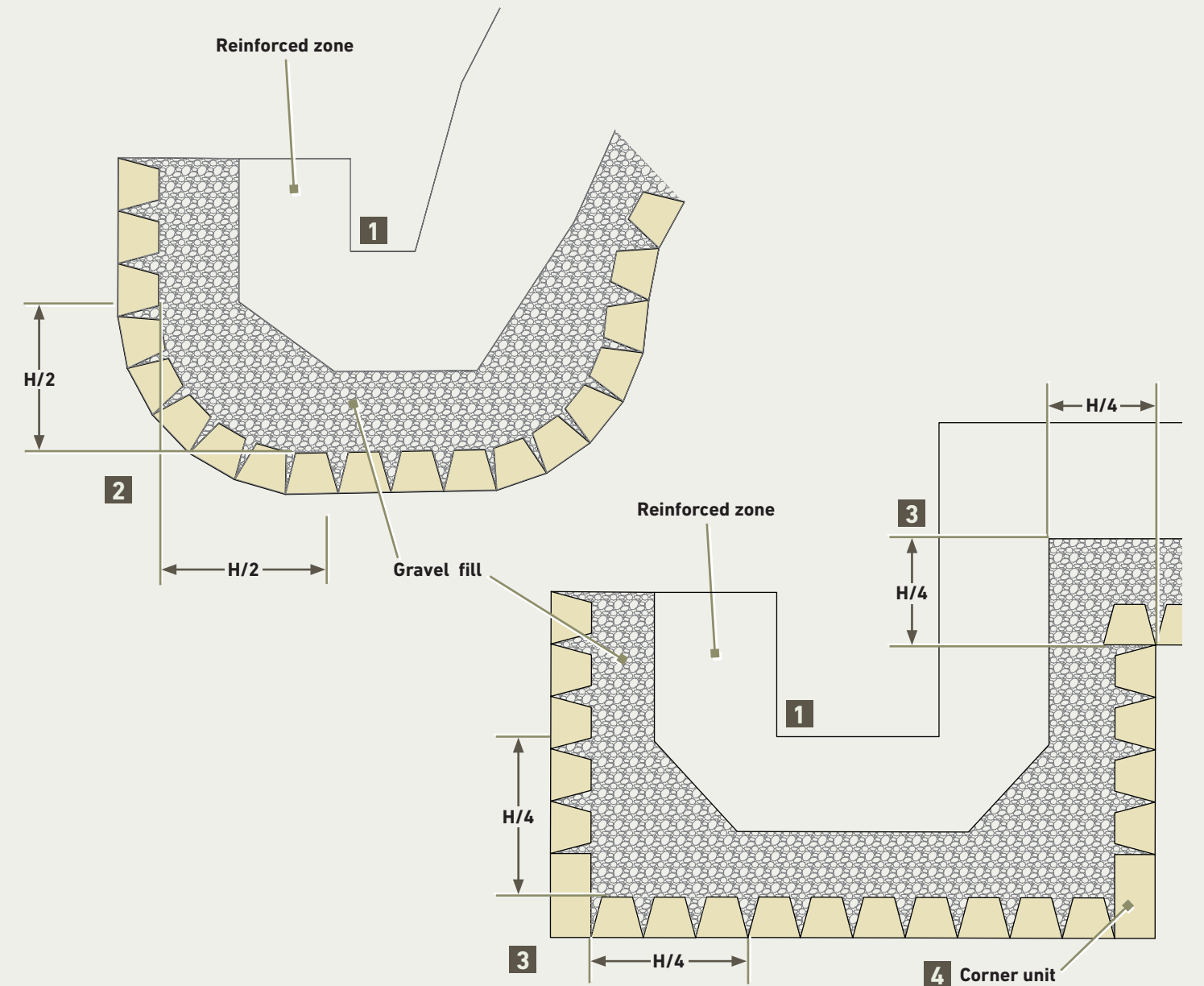
Figure 14 | Geogrid Installation on Curves and Corners
