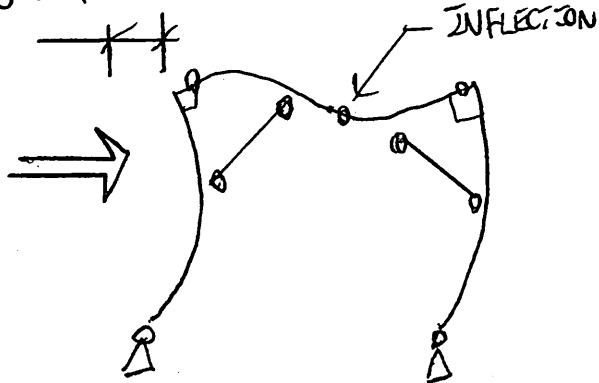
SWAY BUCKLING MODE
