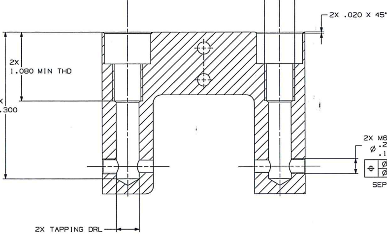
SECTION X-X SCALE 2:1
