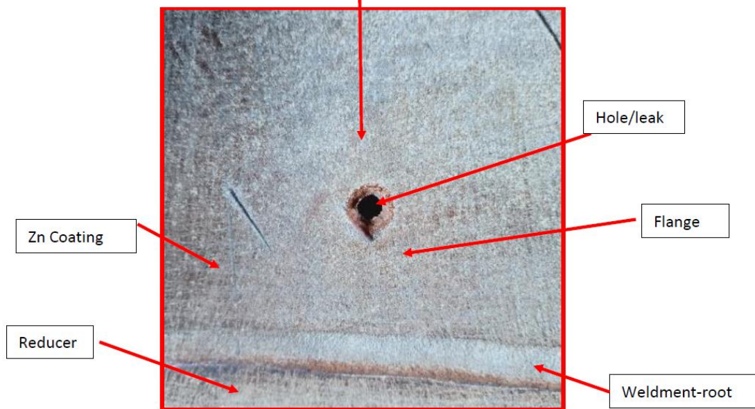
Photo 4: Inner surface corresponds to Photo 3.
