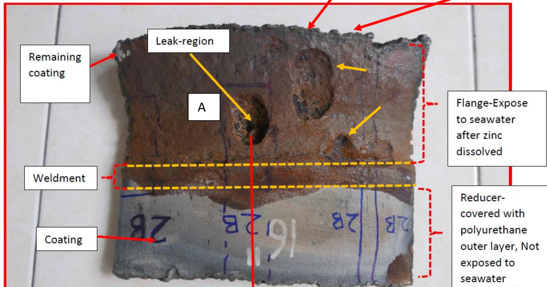
Photo 3: Flange outer surface after cleaning showing pits ( yellow arrows)and pit with hole/leak (A).
