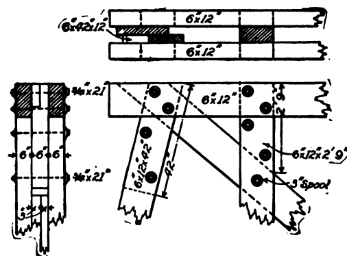
FIG. 3. -CAP AND POST JOINT.
