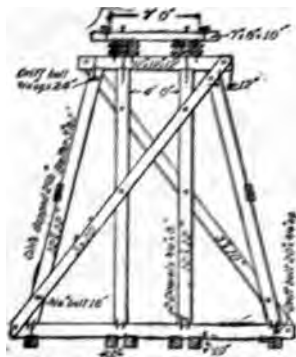
FIG. 1.—CROSS-SECTION.
