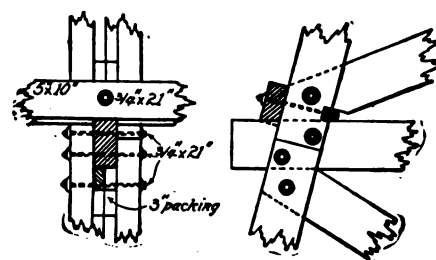
FIG. 4. -POST-SPLICE.
