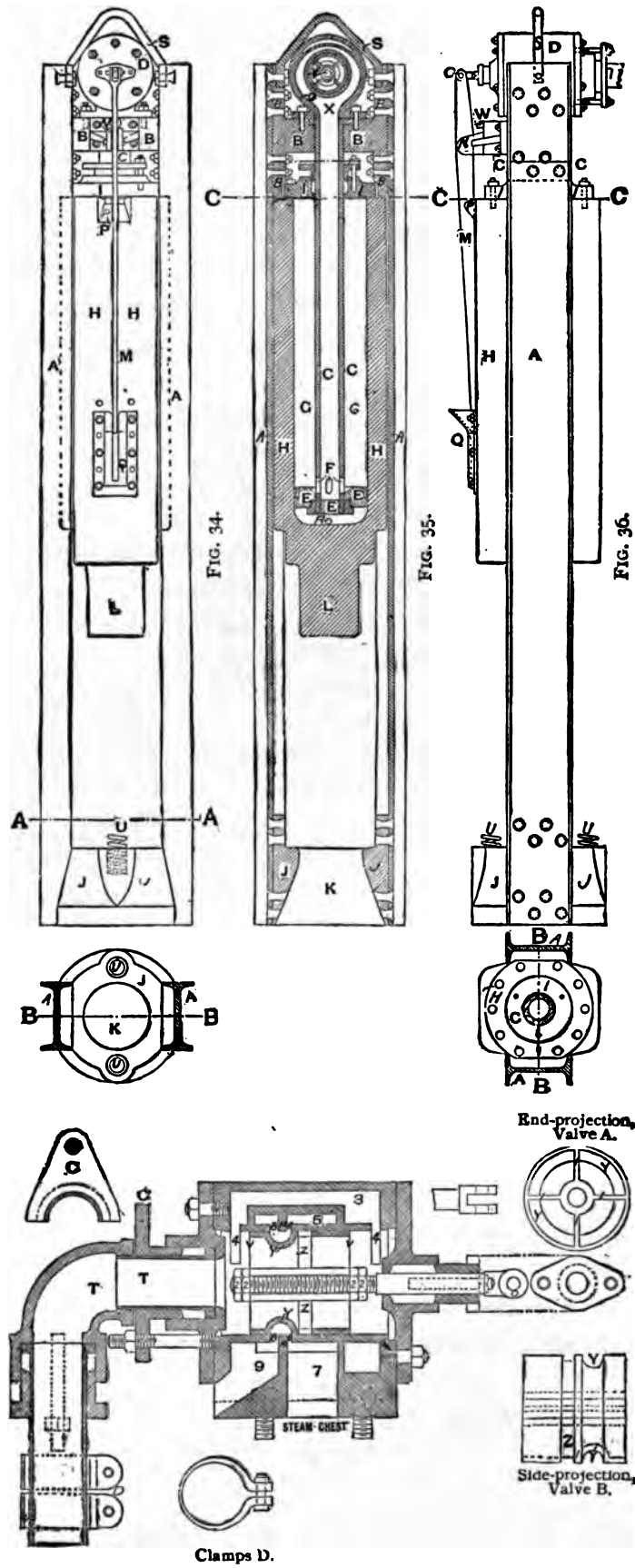
FIGS. 34 to 37.—DETAILS OF CRAM'S STEAM PILE-HAMMER.
