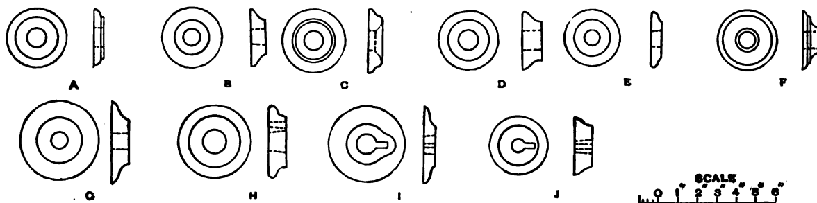
FIG. 131.—CAST-IRON WASHERS.
