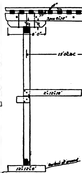
FIG. 2.—ELEVATION.
