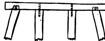
FIG. 21.—FASTENING CAP TO PILES.
