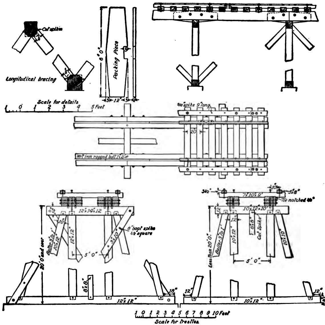
PLATE XL.—STANDARD FRAMED TRETTLES, PENNSYLVANIA RAILROAD.
