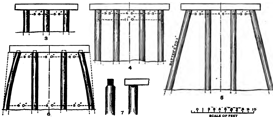
FIGS. 3 TO 7.—PILE-BENTS.
