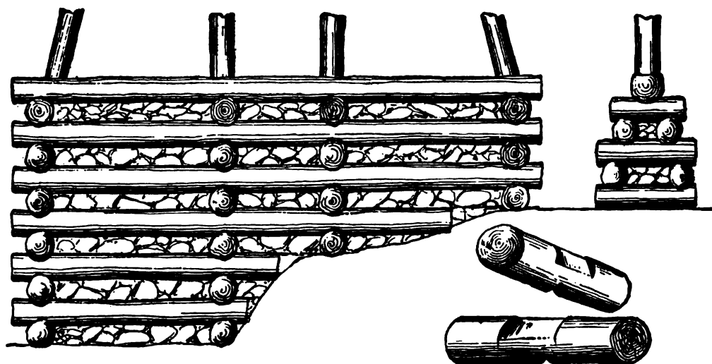
FIG. 41.—CRIB FOUNDATIONS.
