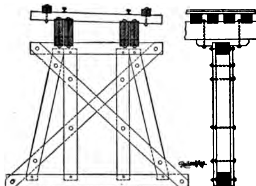
FIG. 125A.—UNEQUAL CORBELS.
