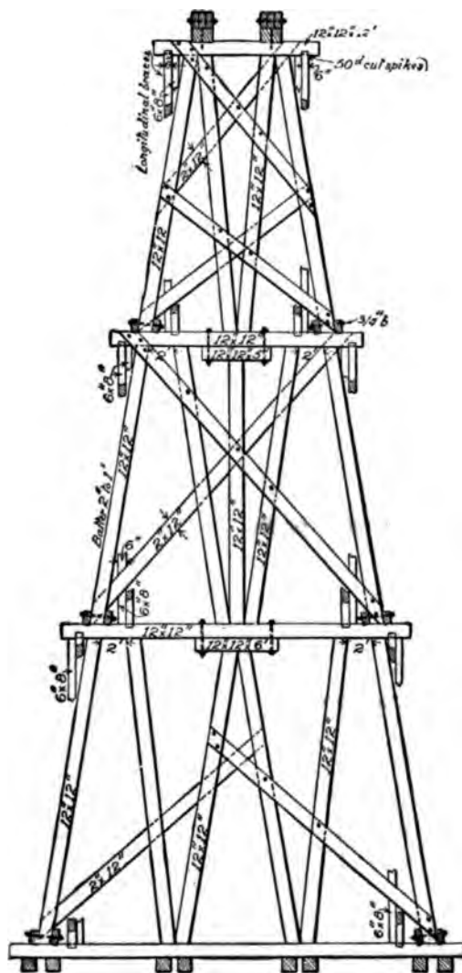
FIG. 1.—CROSS-SECTION.
