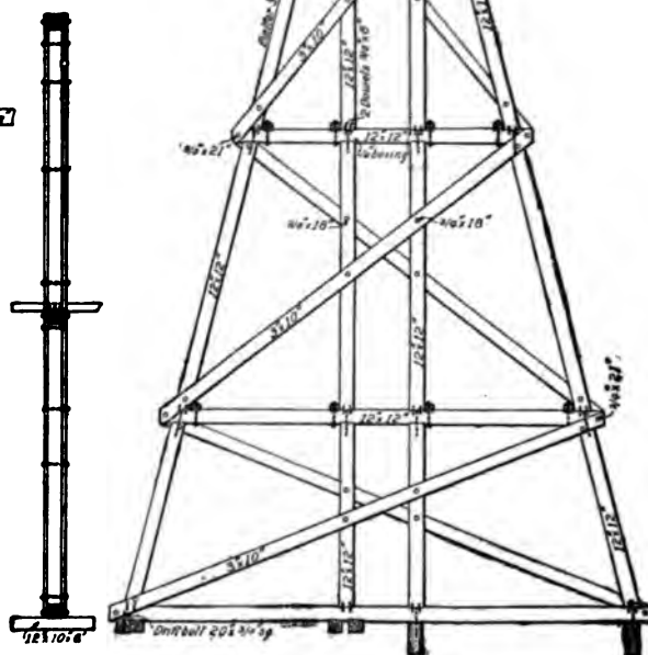
FIG. 7.—TRIPLE-DECK TRESTLE.
