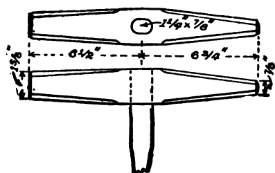
FIG. 134.—SPIKE-MAUL.
