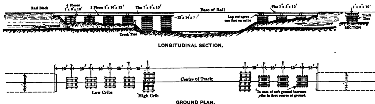
FIG. 159.—SKETCH SHOWING METHOD OF BRIDGING A WASHOUT WITH CRIBS OF TRACK-TIES.
