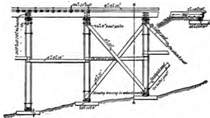
FIG. 2.—ELEVATION.
