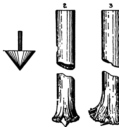
FIG. 11a.—EFFECT OF SHOES ON PILES.
