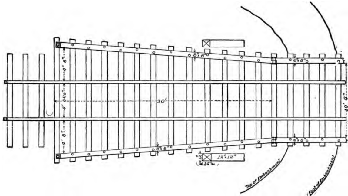
FIG. 118.—EMBANKMENT END OF TRESTLE, SHOWING FLARED GUARD-RAILS AND BUMPING-POSTS.
