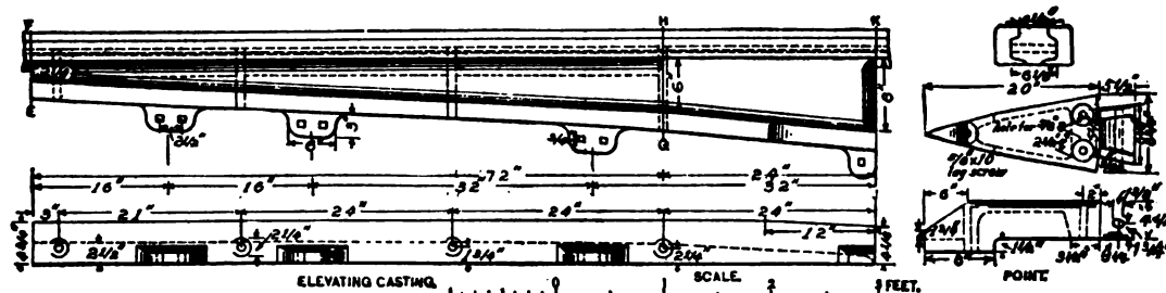
Elevating Casting and Point.
