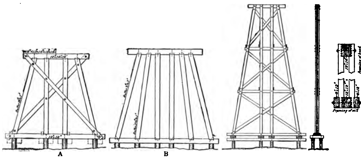
FIG. 1.—FRAMED BENTS.
