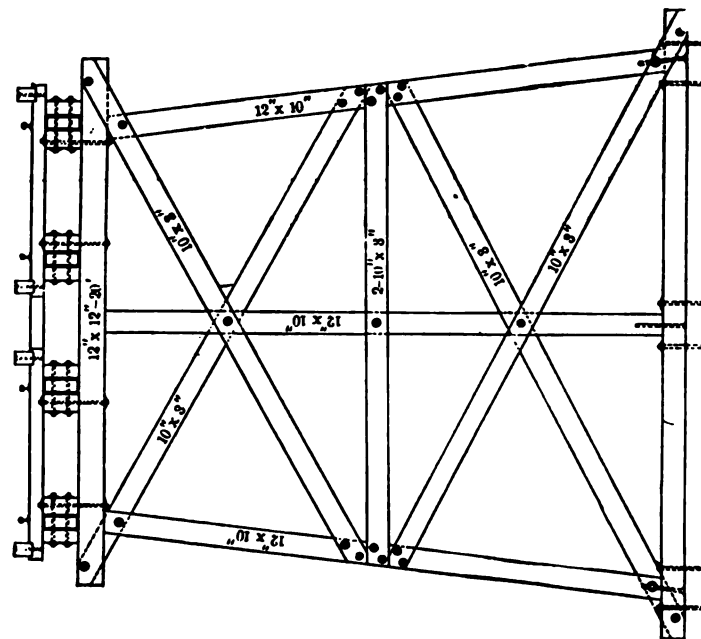
PLATE XLVII.—TRESTLE, BUFFALO & NIAGARA FALLS ELECTRIC RAILWAY.
