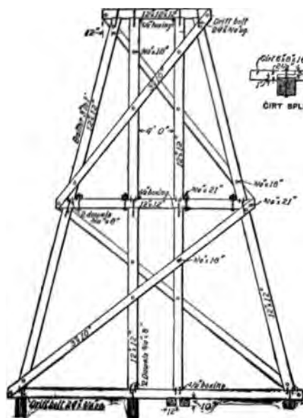
FIG. 6.—DOUBLE-DECK TRESTLE.
