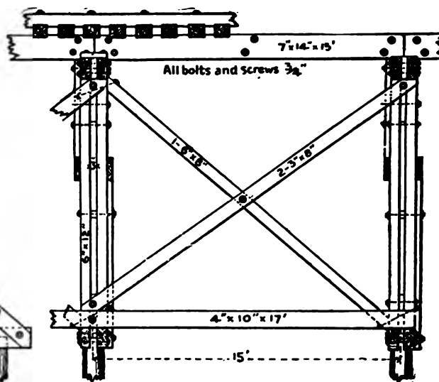
FIG. 2.—ELEVATION.
