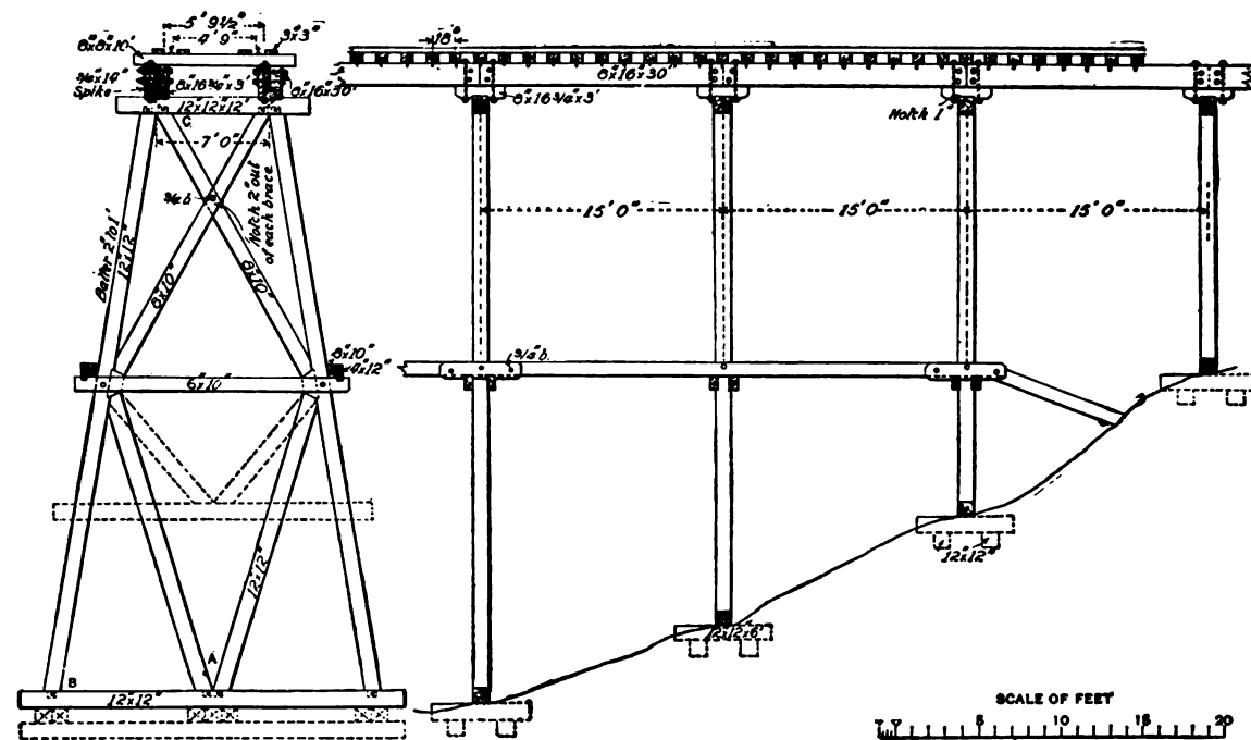
FIG. 1.—GENERAL PLANS.
