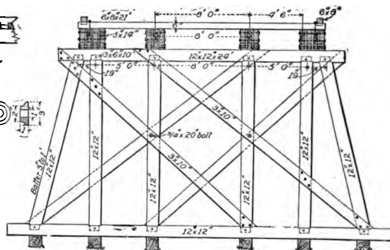
FIG. 2.—CROSS-SECTION.
