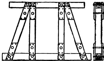
FIG. 50.—PLASTER-JOINTS.
