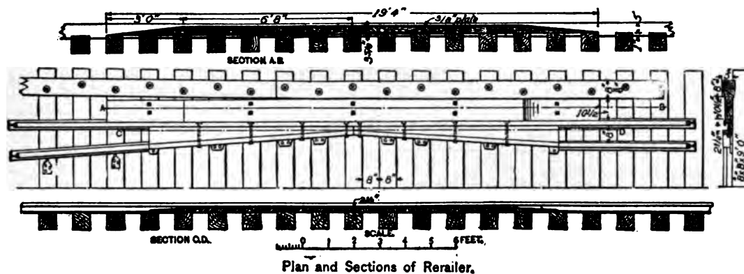
Plan and Sections of Retainer.
