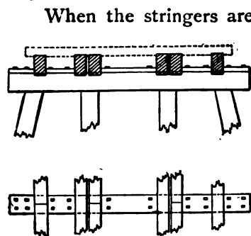
FIG. 99.—STRINGER FASTENING.
