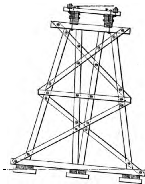
FIG. 125C.—TILTED FRAME TRESTLE.
