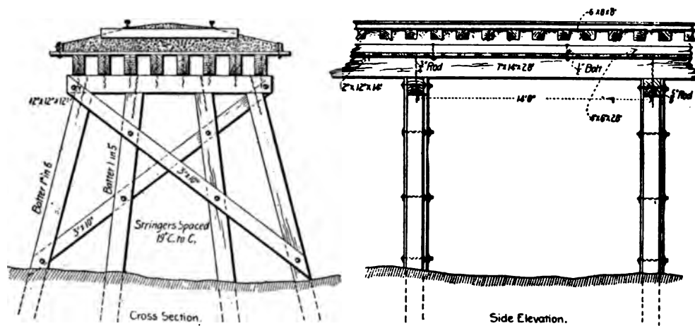
PLATE VIII A.—TRETTLE WITH BALLASTED FLOOR, HOUSTON & TEXAS CENTRAL R. R.
