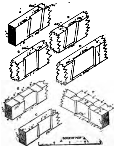
FIG. 5.—DETAILS OF WALLS AND GIRTS.
