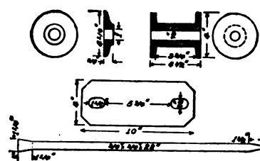
FIG. 3.—IRON DETAILS.
