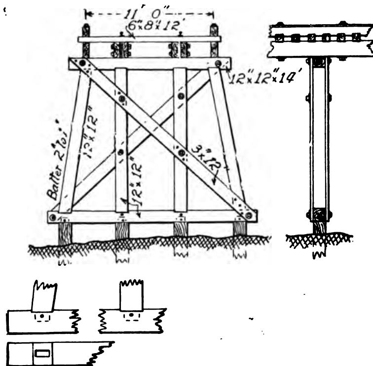
PLATE X.—STANDARD FRAMED TRESTLE, CHICAGO & WEST MICHIGAN RAILWAY.
