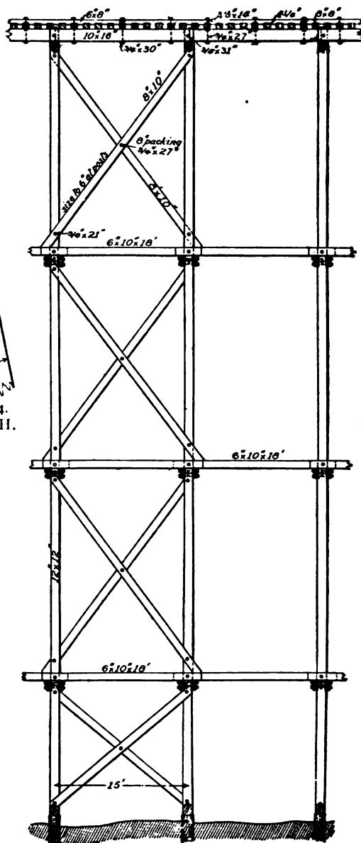
FIG. 2.—ELEVATION.
