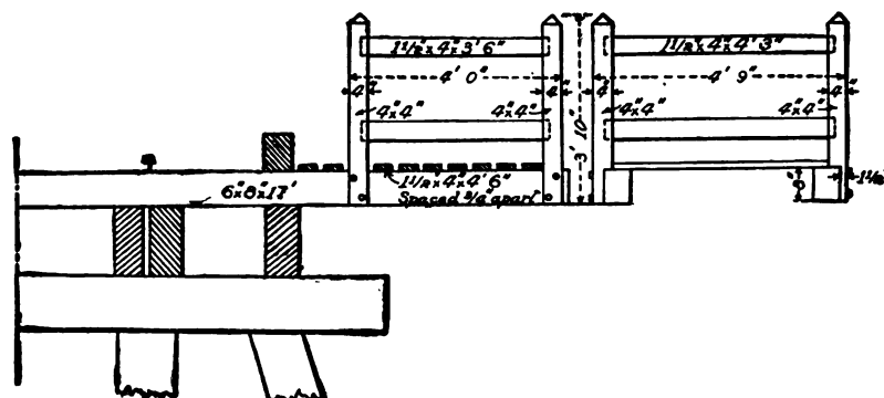
FIG. 133.—REFUGE-BAY.
