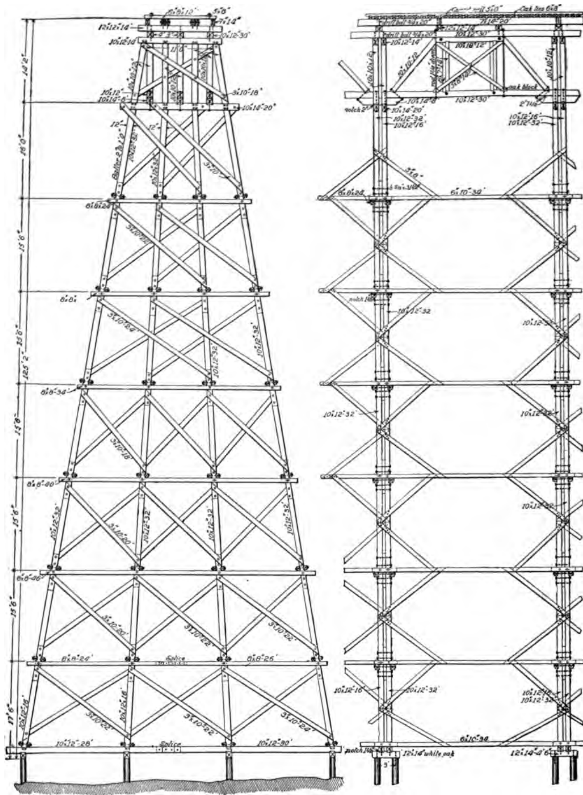
PLATE XXXIV.—FRAMED TRESTLE, ST. PAUL, MINNEAPOLIS & MANITOBA RAILROAD.
