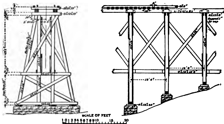
FIG. 1.—CROSS-SECTION.
