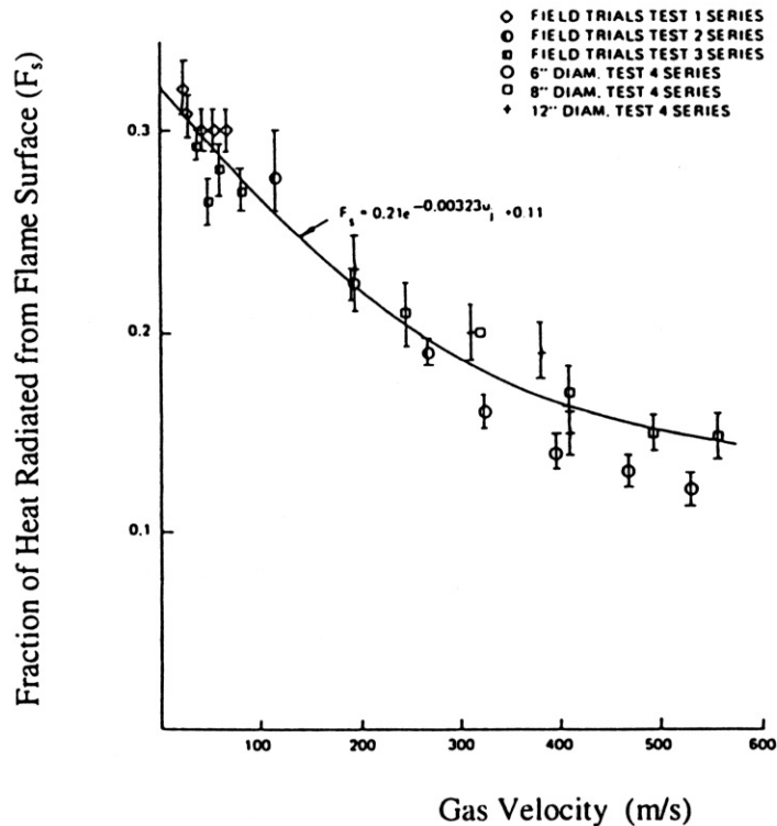
Figure 6 – Fraction of heat radiated from the flame surface verses gas velocity for pipe flares. The vertical bars represent the standard deviation at each point (Chamberlain, 1987).
