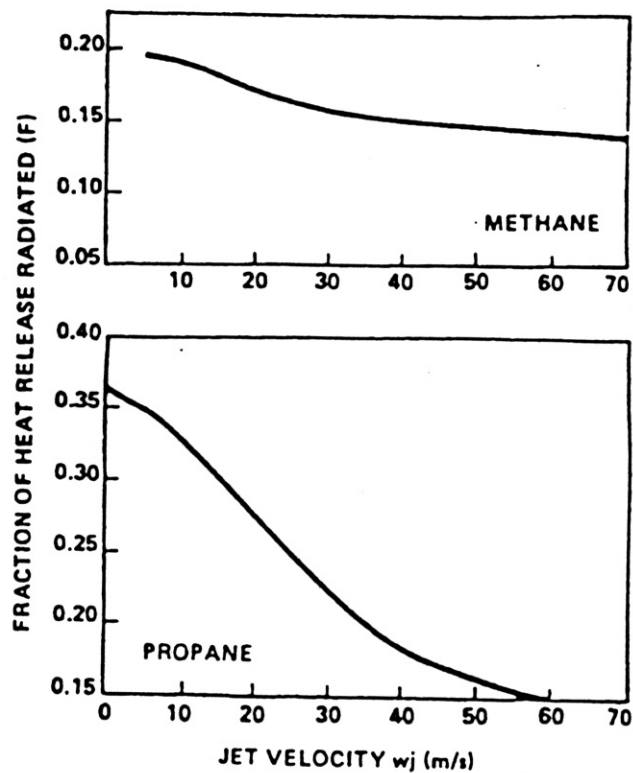
Figure 8 - Effect of jet exit velocity on the fraction of heat radiated in the absence of a cross-wind (taken from Barnwell and Marshall, 1984).
