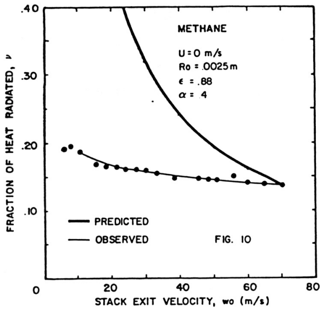
Figures 1 and 2 – Comparison between the predicted and observed fractions of heat radiated as a function of stack exit velocity for calm conditions (Leahey et al., 1979).
