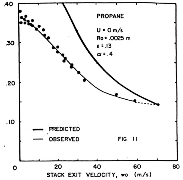
Figures 1 and 2 – Comparison between the predicted and observed fractions of heat radiated as a function of stack exit velocity for calm conditions (Leahey et al., 1979).
