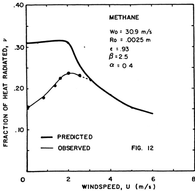
Figures 3 and 4 – Comparison between the predicted and observed fractions of heat radiated as a function of wind speed (Leahey et al., 1979).
