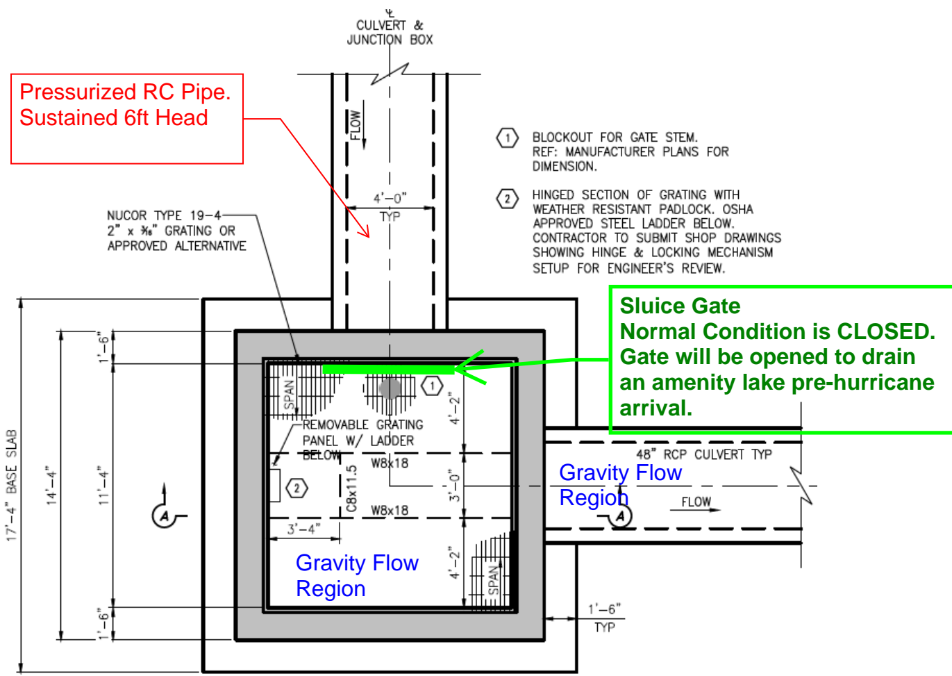
PLAN VIEW – PROPOSED SQUARE JUNCTION BOX
