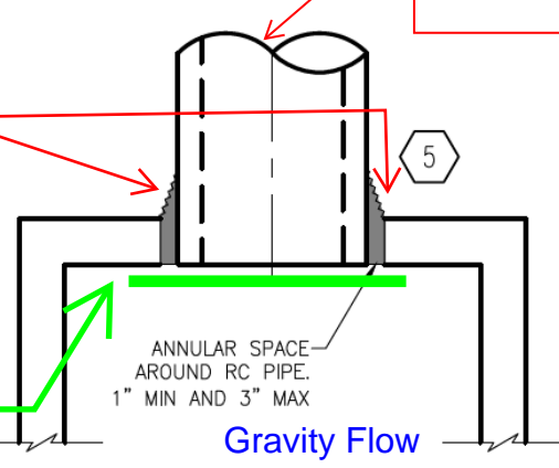
TYPICAL HALF PLAN – PIPE TO WALL CONNECTION
