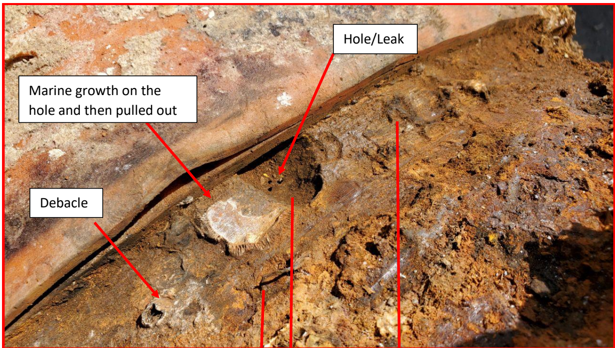
Photo 1: Showing the affected locations before the the polyurethane outer cover and the the deposit on the flange were removed.
