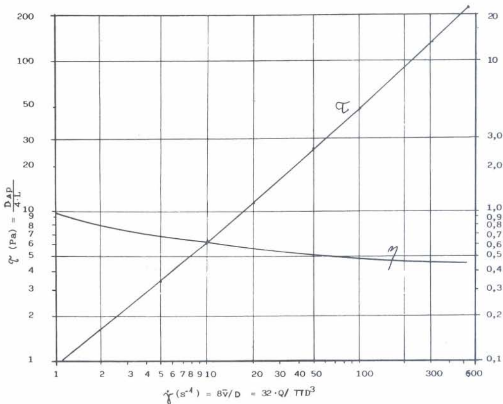
Fig. 2. Flow diagram: \tau = D\Delta p/4L (Pa) - shear stress, \dot{\gamma} = dv/dr = 8\bar{v}/D = 32Q/\pi D^3 ( s^{-1} ) - shear rate, \eta_a - apparent viscosity (Pa·s)
