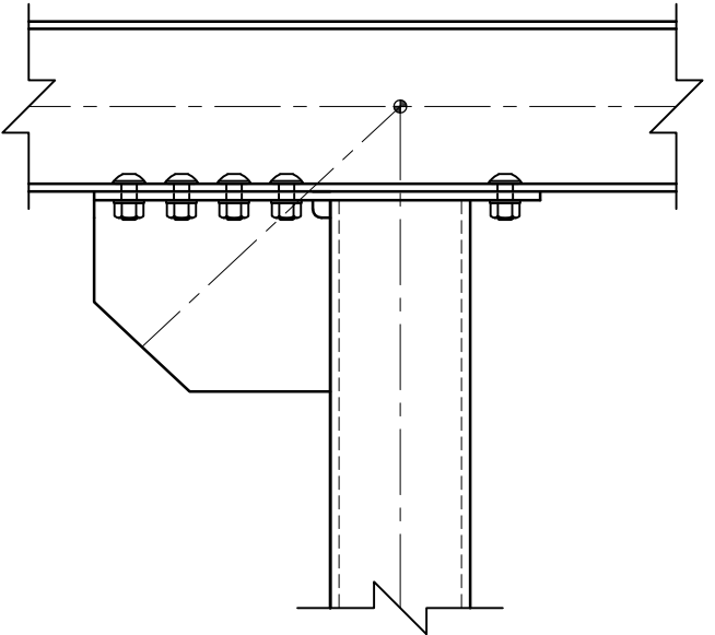
SECTION 2-2
