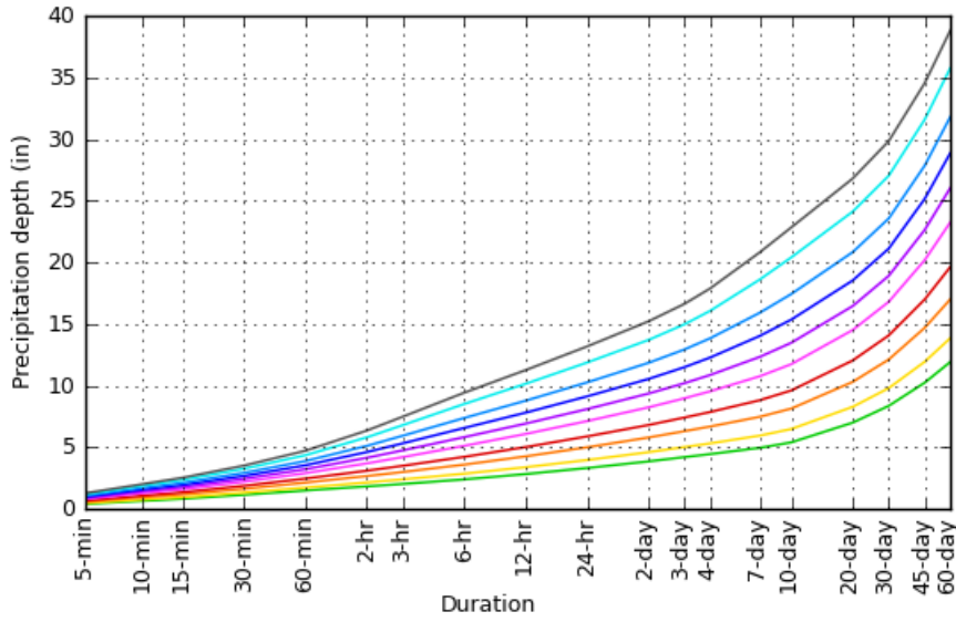
PDS-based depth-duration-frequency (DDF) curves Latitude: 33.2191°, Longitude: -97.0024°
