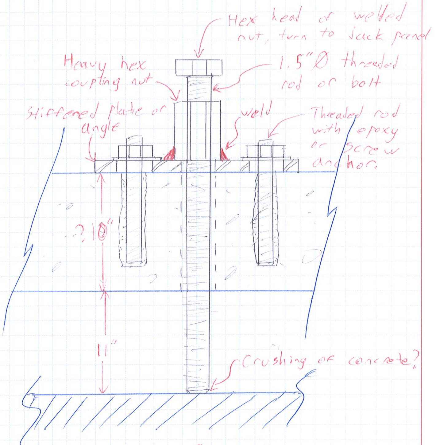
Roof Jacking Bolt (Typ. 3 places)
