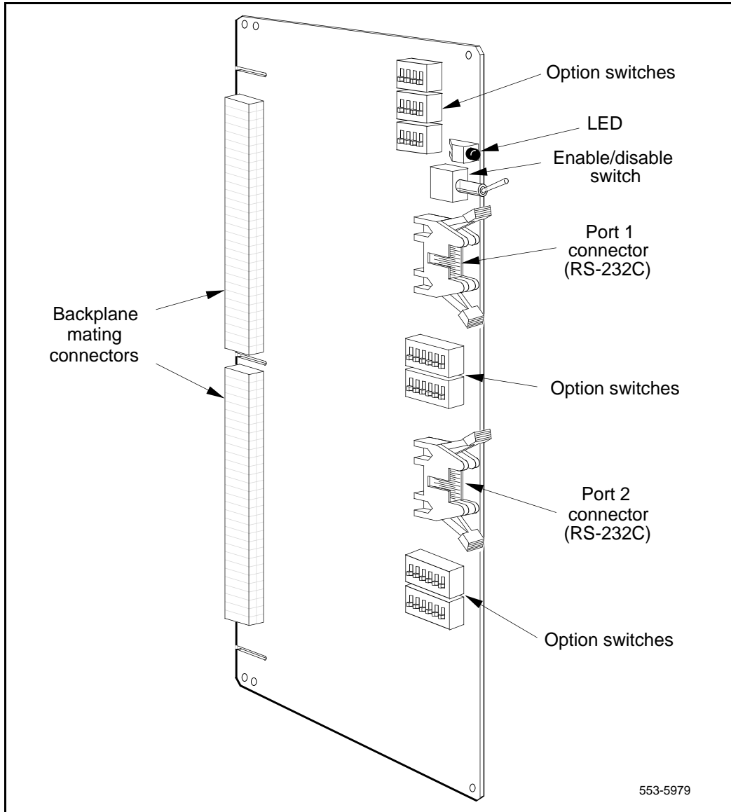
Figure 1 NT8D41AA SDI paddle board
