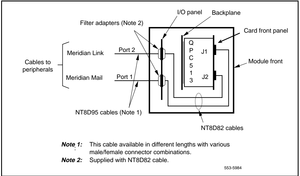
Figure 16 QPC513 ESDI card cabling
