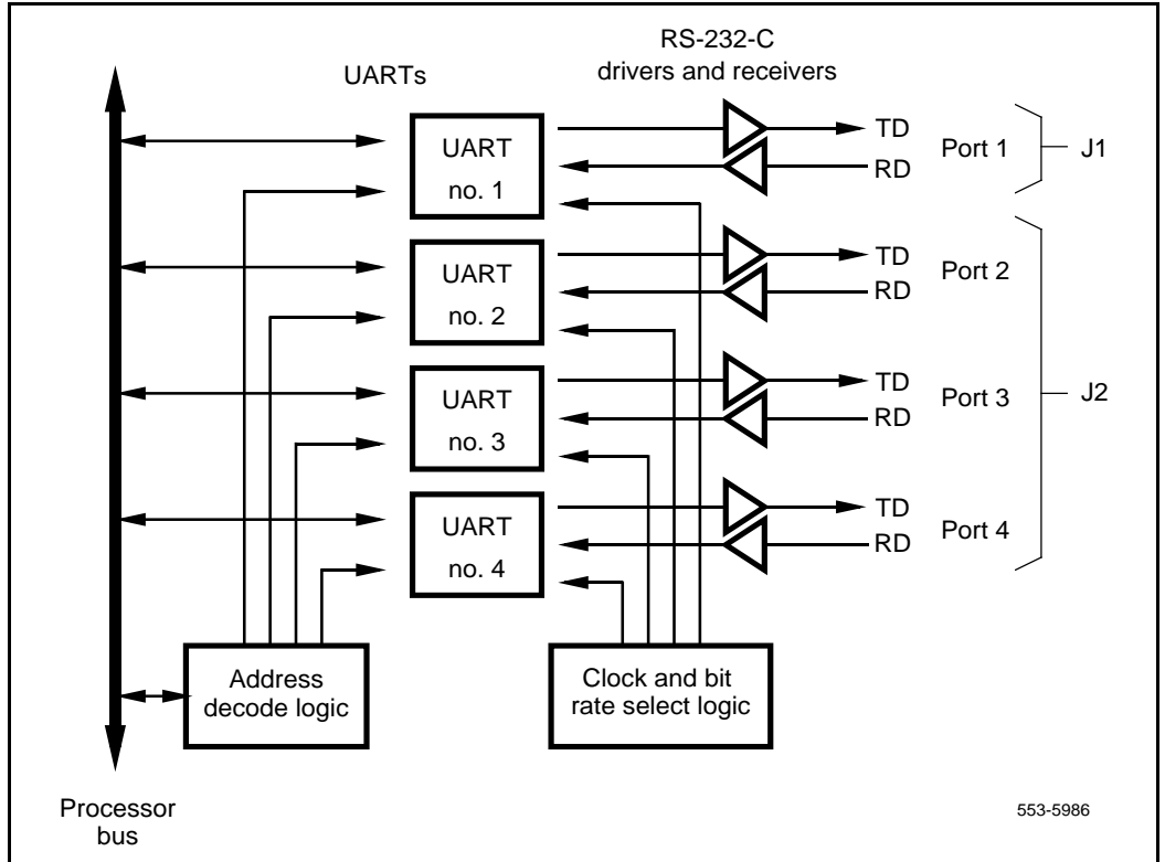
Figure 9 QPC841 QSDI Card block diagram
