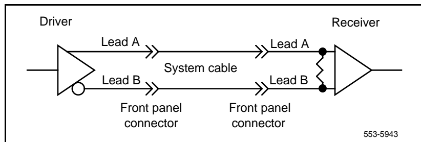
Figure 14 Typical high-speed interface line driver and receiver
