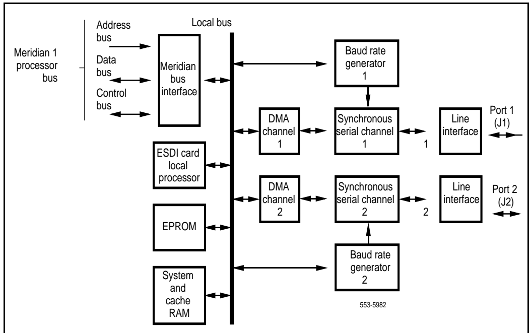
Figure 13 ESDI card block diagram
